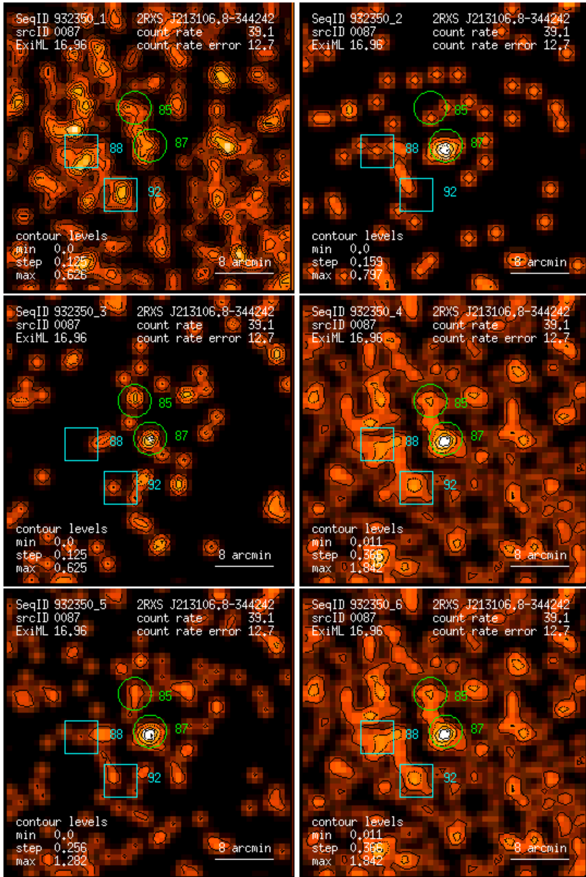
Figure 87: RASS 932350: detection 0087: band rate images, Gaussian filter: (1) PSPC channels 11 – 41, (2) 52 – 90, (3) 91 – 201, (4) 11 – 235, (5) 52 – 201, (6) 11 – 201. Broad band rates in counts/ks. Band rate contour levels in counts/ks/arcmin 2 .
