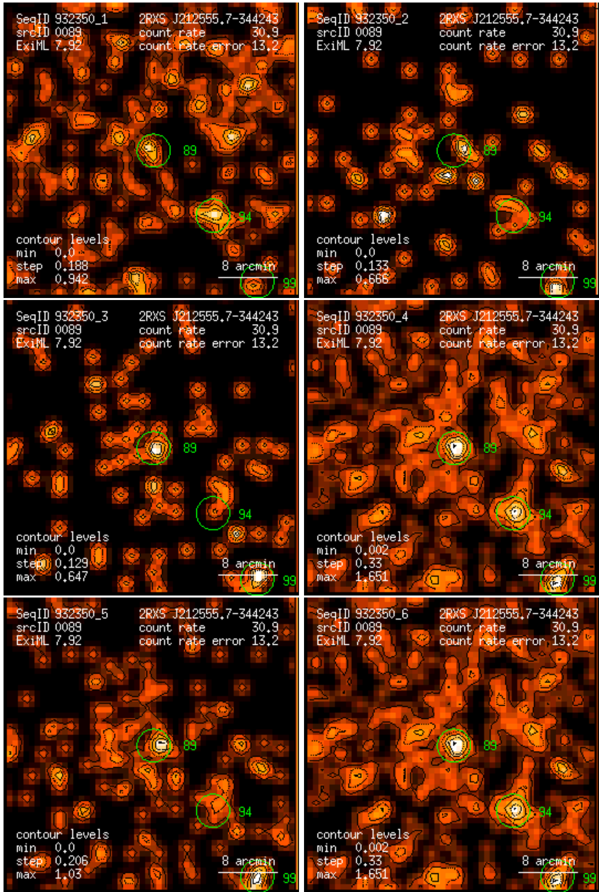
Figure 89: RASS 932350: detection 0089: band rate images, Gaussian filter: (1) PSPC channels 11 – 41, (2) 52 – 90, (3) 91 – 201, (4) 11 – 235, (5) 52 – 201, (6) 11 – 201. Broad band rates in counts/ks. Band rate contour levels in counts/ks/arcmin 2 .
