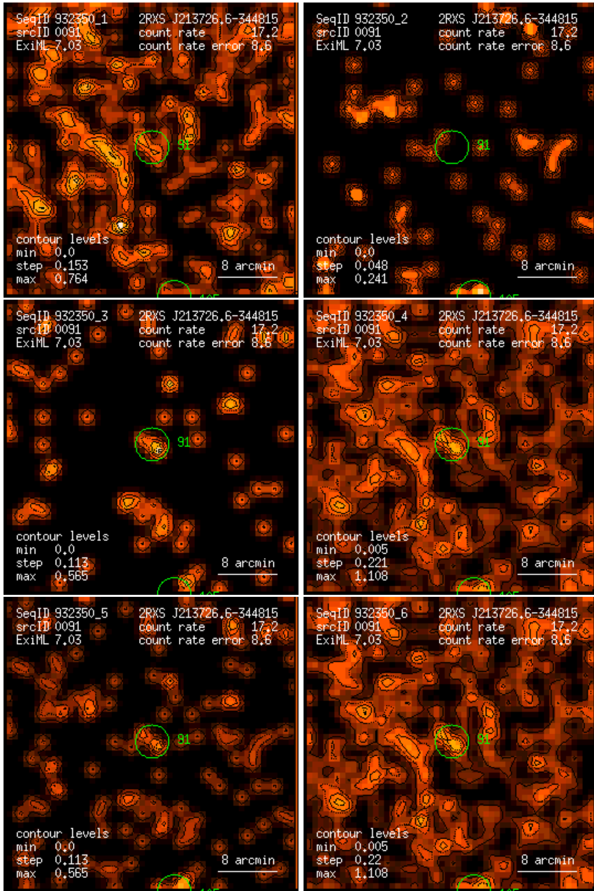
Figure 91: RASS 932350: detection 0091: band rate images, Gaussian filter: (1) PSPC channels 11 – 41, (2) 52 – 90, (3) 91 – 201, (4) 11 – 235, (5) 52 – 201, (6) 11 – 201. Broad band rates in counts/ks. Band rate contour levels in counts/ks/arcmin 2 .
