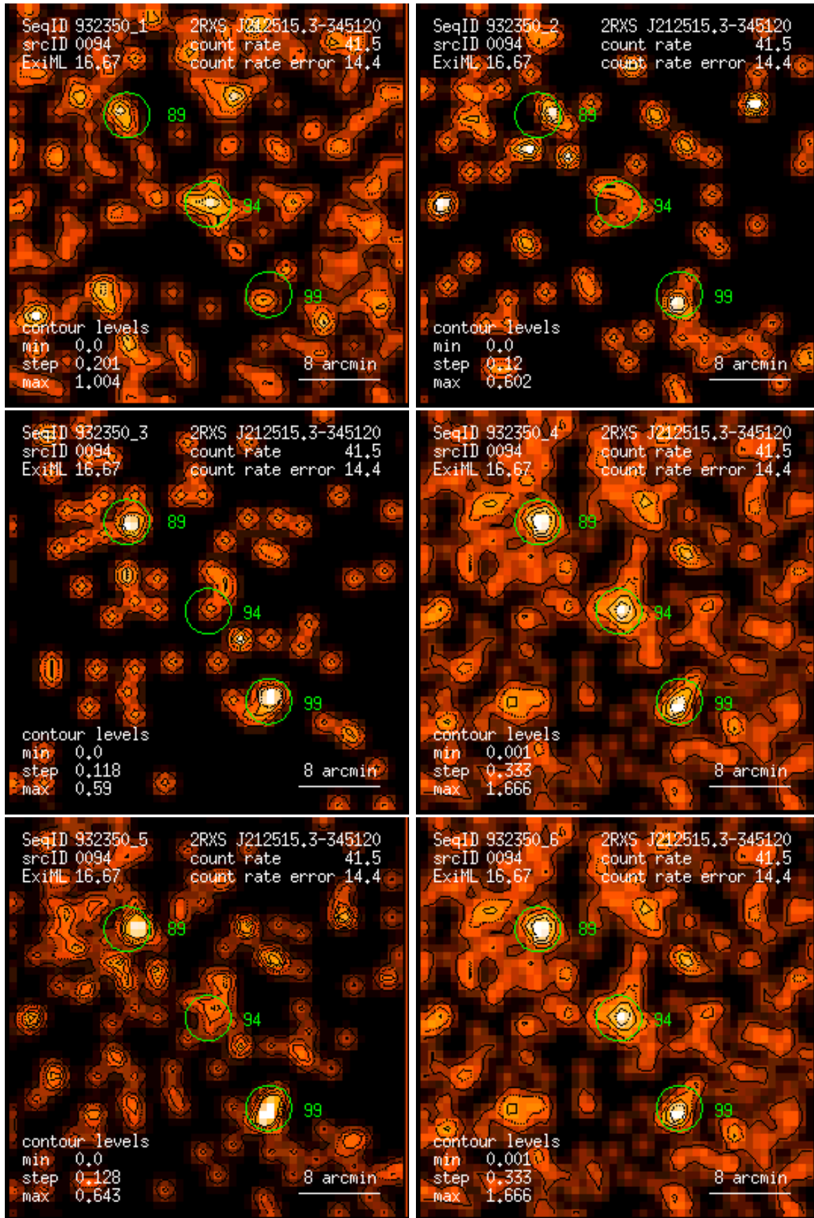
Figure 94: RASS 932350: detection 0094: band rate images, Gaussian filter: (1) PSPC channels 11 – 41, (2) 52 – 90, (3) 91 – 201, (4) 11 – 235, (5) 52 – 201, (6) 11 – 201. Broad band rates in counts/ks. Band rate contour levels in counts/ks/arcmin 2 .
