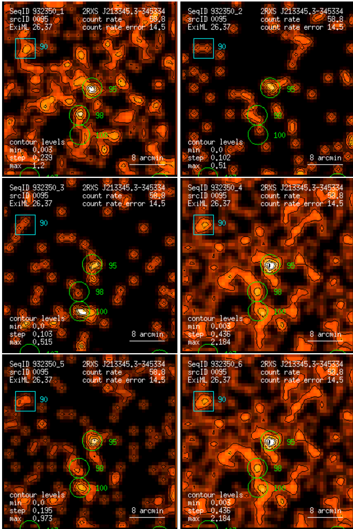
Figure 95: RASS 932350: detection 0095: band rate images, Gaussian filter: (1) PSPC channels 11 – 41, (2) 52 – 90, (3) 91 – 201, (4) 11 – 235, (5) 52 – 201, (6) 11 – 201. Broad band rates in counts/ks. Band rate contour levels in counts/ks/arcmin 2 .
