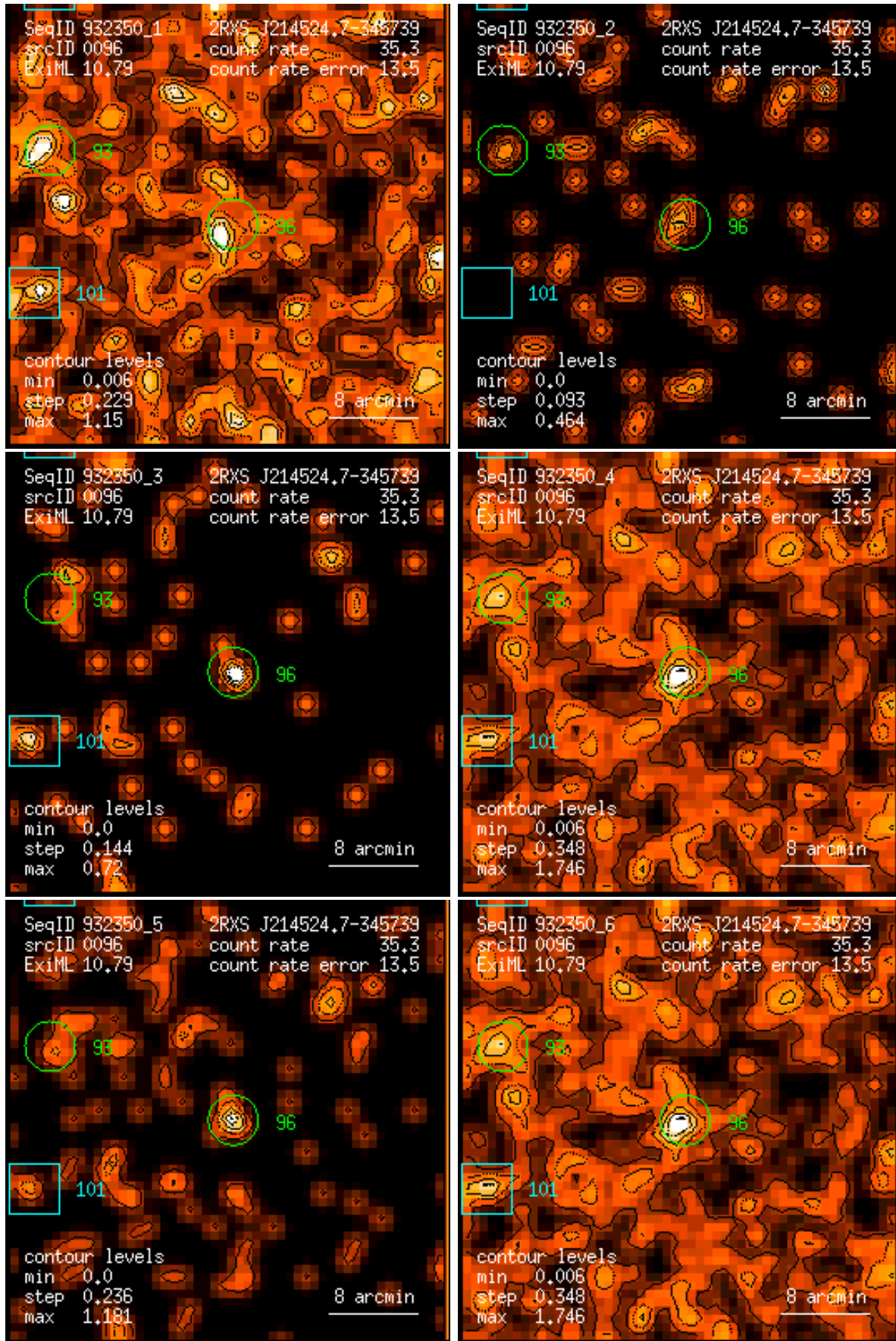
Figure 96: RASS 932350: detection 0096: band rate images, Gaussian filter: (1) PSPC channels 11 – 41, (2) 52 – 90, (3) 91 – 201, (4) 11 – 235, (5) 52 – 201, (6) 11 – 201. Broad band rates in counts/ks. Band rate contour levels in counts/ks/arcmin 2 .
