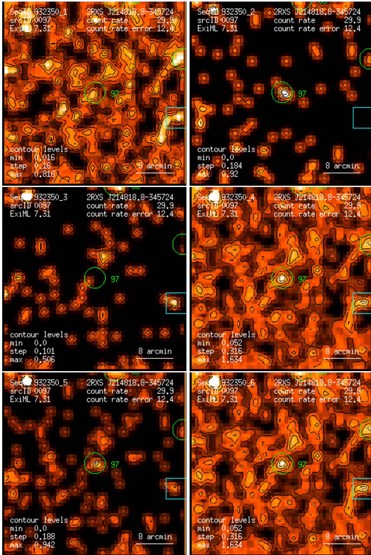
Figure 97: RASS 932350: detection 0097: band rate images, Gaussian filter: (1) PSPC channels 11 – 41, (2) 52 – 90, (3) 91 – 201, (4) 11 – 235, (5) 52 – 201, (6) 11 – 201. Broad band rates in counts/ks. Band rate contour levels in counts/ks/arcmin 2 .
