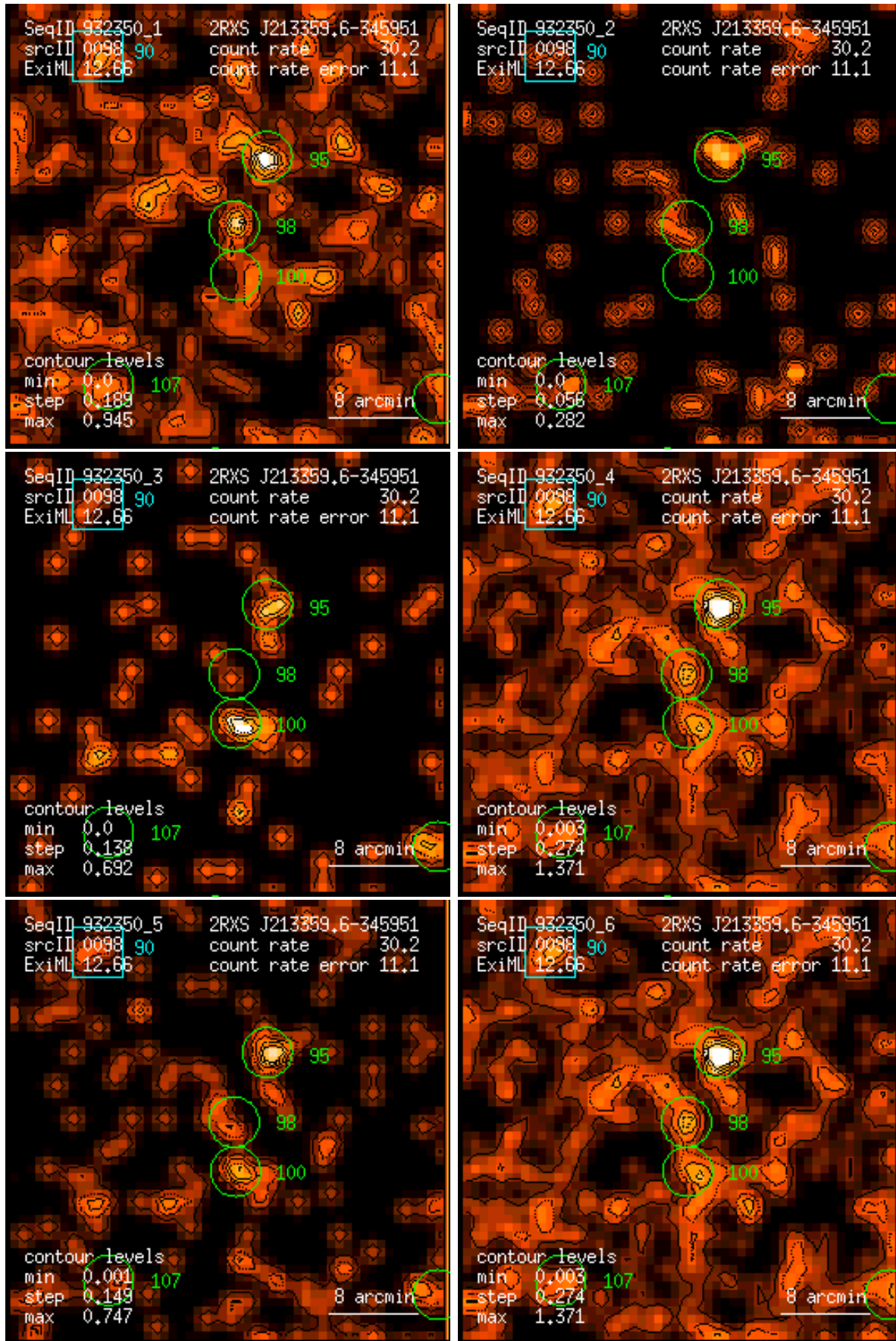
Figure 98: RASS 932350: detection 0098: band rate images, Gaussian filter: (1) PSPC channels 11 – 41, (2) 52 – 90, (3) 91 – 201, (4) 11 – 235, (5) 52 – 201, (6) 11 – 201. Broad band rates in counts/ks. Band rate contour levels in counts/ks/arcmin 2 .
