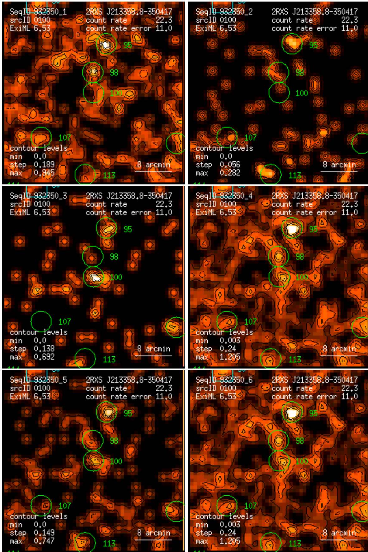
Figure 100: RASS 932350: detection 0100: band rate images, Gaussian filter: (1) PSPC channels 11 – 41, (2) 52 – 90, (3) 91 – 201, (4) 11 – 235, (5) 52 – 201, (6) 11 – 201. Broad band rates in counts/ks. Band rate contour levels in counts/ks/arcmin 2 .
