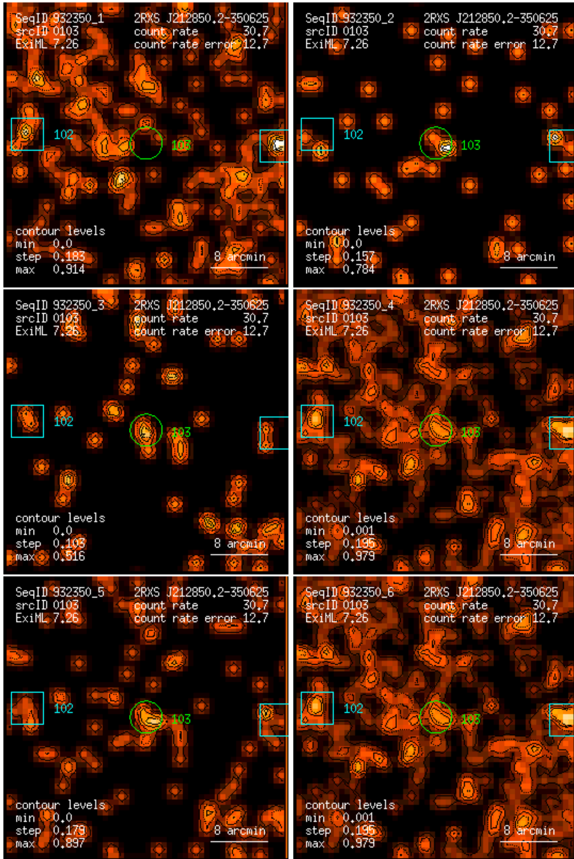
Figure 103: RASS 932350: detection 0103: band rate images, Gaussian filter: (1) PSPC channels 11 – 41, (2) 52 – 90, (3) 91 – 201, (4) 11 – 235, (5) 52 – 201, (6) 11 – 201. Broad band rates in counts/ks. Band rate contour levels in counts/ks/arcmin 2 .
