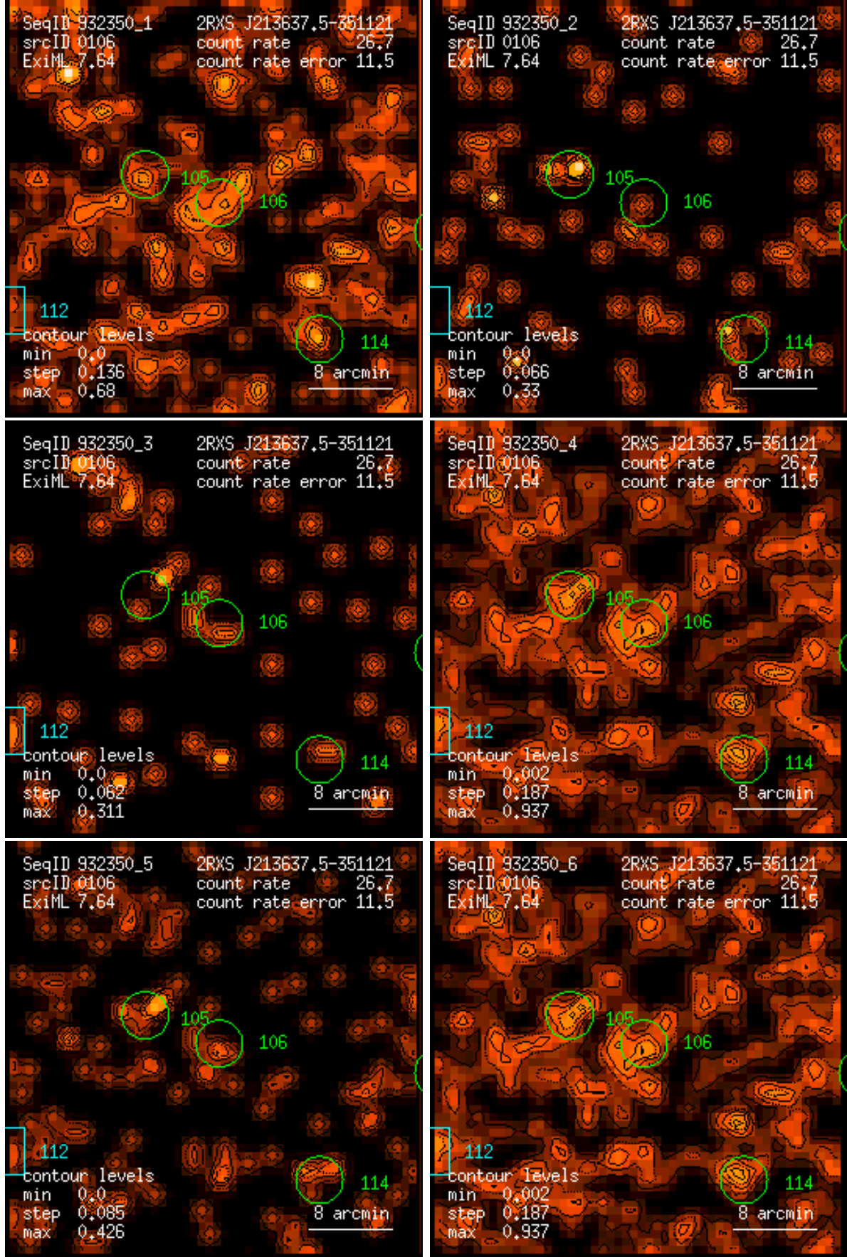
Figure 106: RASS 932350: detection 0106: band rate images, Gaussian filter: (1) PSPC channels 11 – 41, (2) 52 – 90, (3) 91 – 201, (4) 11 – 235, (5) 52 – 201, (6) 11 – 201. Broad band rates in counts/ks. Band rate contour levels in counts/ks/arcmin 2 .
