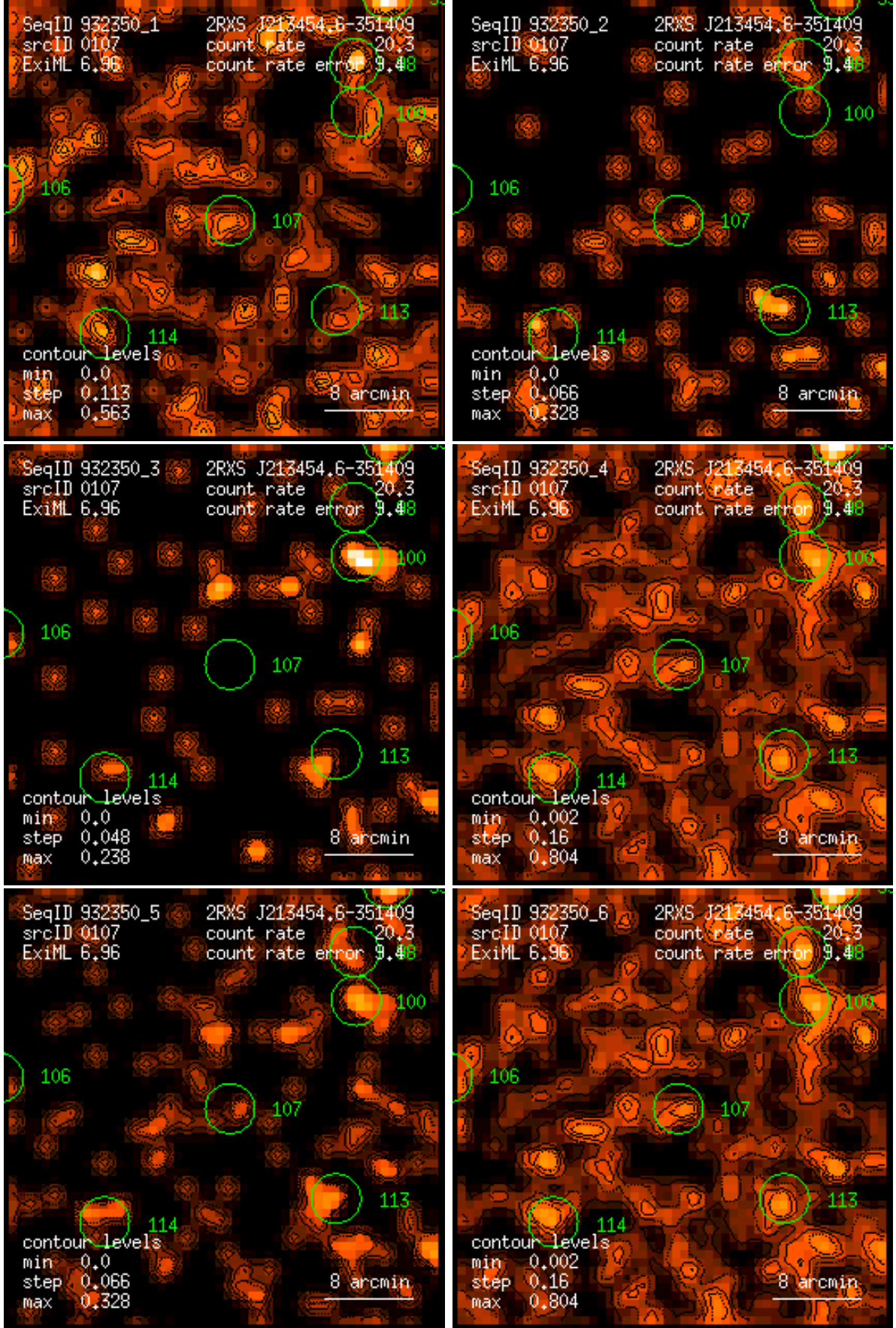
Figure 107: RASS 932350: detection 0107: band rate images, Gaussian filter: (1) PSPC channels 11 – 41, (2) 52 – 90, (3) 91 – 201, (4) 11 – 235, (5) 52 – 201, (6) 11 – 201. Broad band rates in counts/ks. Band rate contour levels in counts/ks/arcmin 2 .
