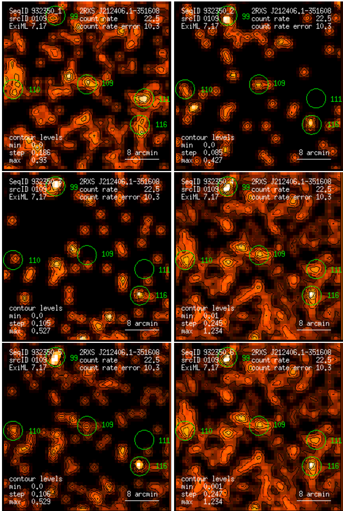
Figure 109: RASS 932350: detection 0109: band rate images, Gaussian filter: (1) PSPC channels 11 – 41, (2) 52 – 90, (3) 91 – 201, (4) 11 – 235, (5) 52 – 201, (6) 11 – 201. Broad band rates in counts/ks. Band rate contour levels in counts/ks/arcmin 2 .
