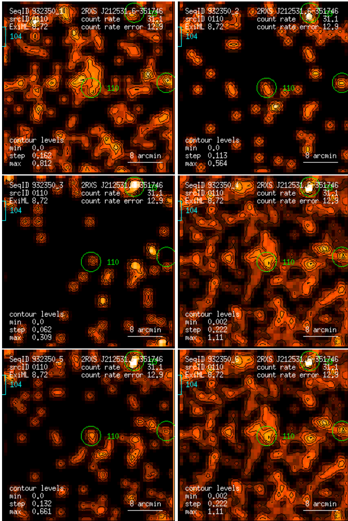
Figure 110: RASS 932350: detection 0110: band rate images, Gaussian filter: (1) PSPC channels 11 – 41, (2) 52 – 90, (3) 91 – 201, (4) 11 – 235, (5) 52 – 201, (6) 11 – 201. Broad band rates in counts/ks. Band rate contour levels in counts/ks/arcmin 2 .
