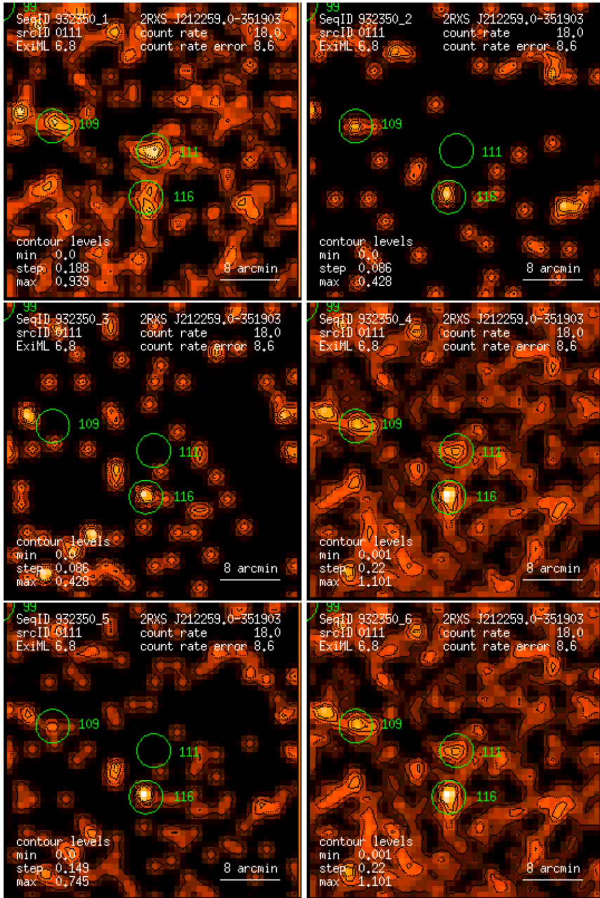
Figure 111: RASS 932350: detection 0111: band rate images, Gaussian filter: (1) PSPC channels 11 – 41, (2) 52 – 90, (3) 91 – 201, (4) 11 – 235, (5) 52 – 201, (6) 11 – 201. Broad band rates in counts/ks. Band rate contour levels in counts/ks/arcmin 2 .
