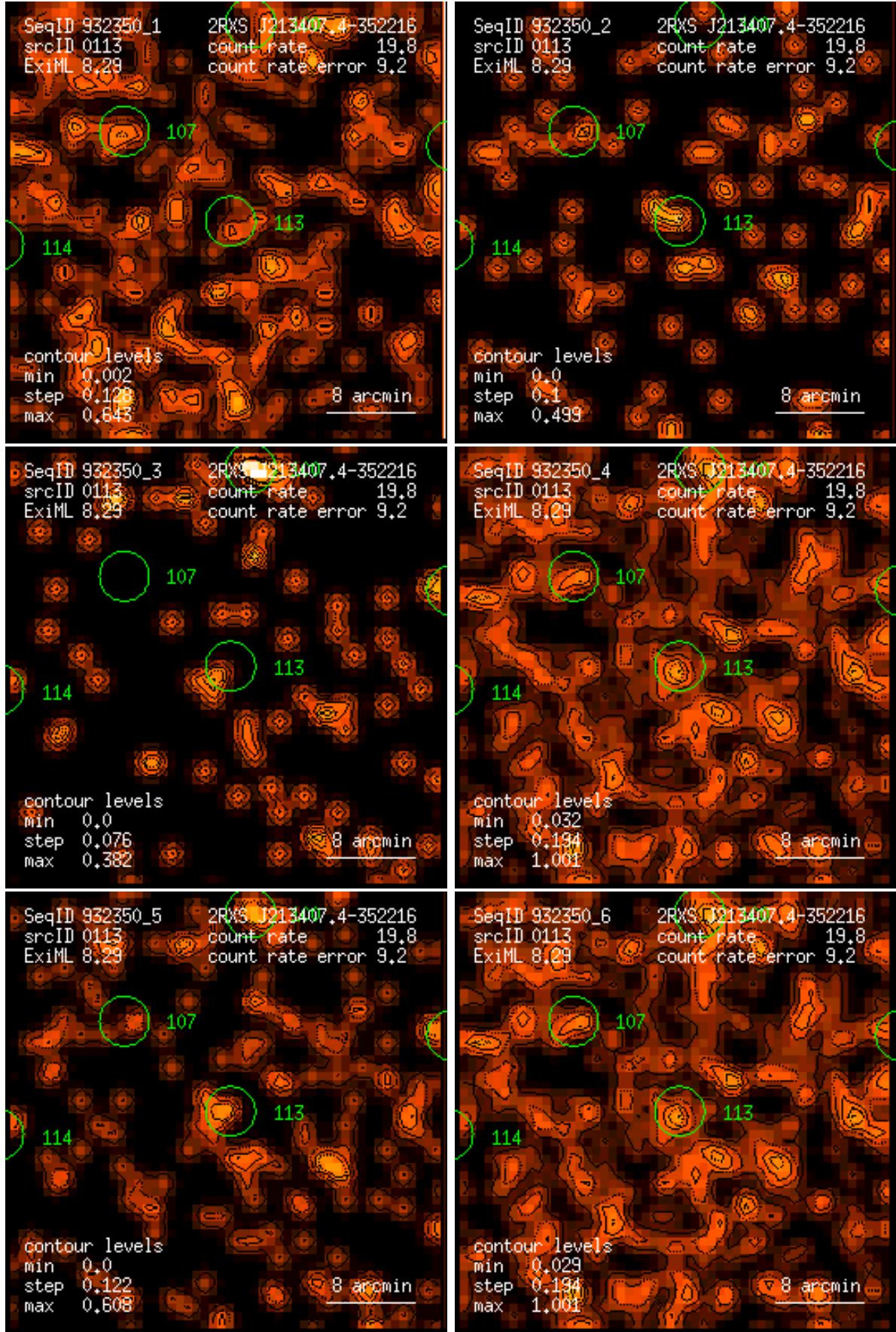
Figure 113: RASS 932350: detection 0113: band rate images, Gaussian filter: (1) PSPC channels 11 – 41, (2) 52 – 90, (3) 91 – 201, (4) 11 – 235, (5) 52 – 201, (6) 11 – 201. Broad band rates in counts/ks. Band rate contour levels in counts/ks/arcmin 2 .
