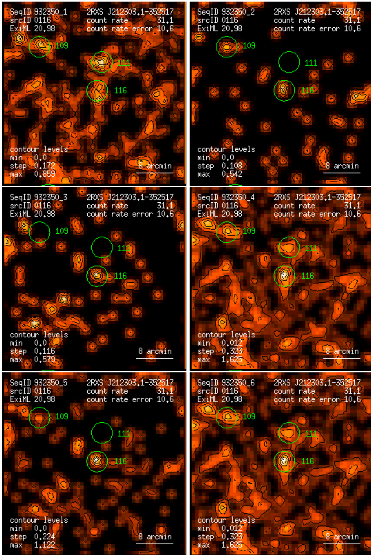
Figure 116: RASS 932350: detection 0116: band rate images, Gaussian filter: (1) PSPC channels 11 – 41, (2) 52 – 90, (3) 91 – 201, (4) 11 – 235, (5) 52 – 201, (6) 11 – 201. Broad band rates in counts/ks. Band rate contour levels in counts/ks/arcmin 2 .
