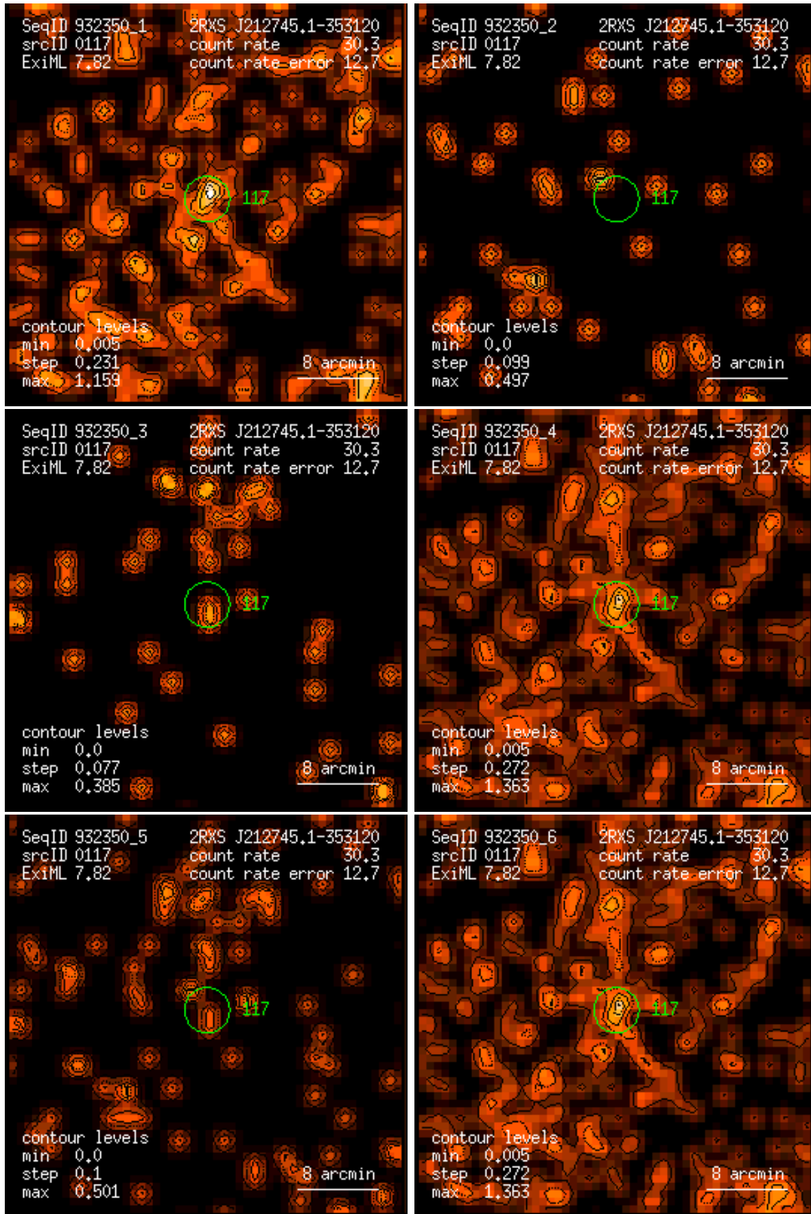
Figure 117: RASS 932350: detection 0117: band rate images, Gaussian filter: (1) PSPC channels 11 – 41, (2) 52 – 90, (3) 91 – 201, (4) 11 – 235, (5) 52 – 201, (6) 11 – 201. Broad band rates in counts/ks. Band rate contour levels in counts/ks/arcmin 2 .
