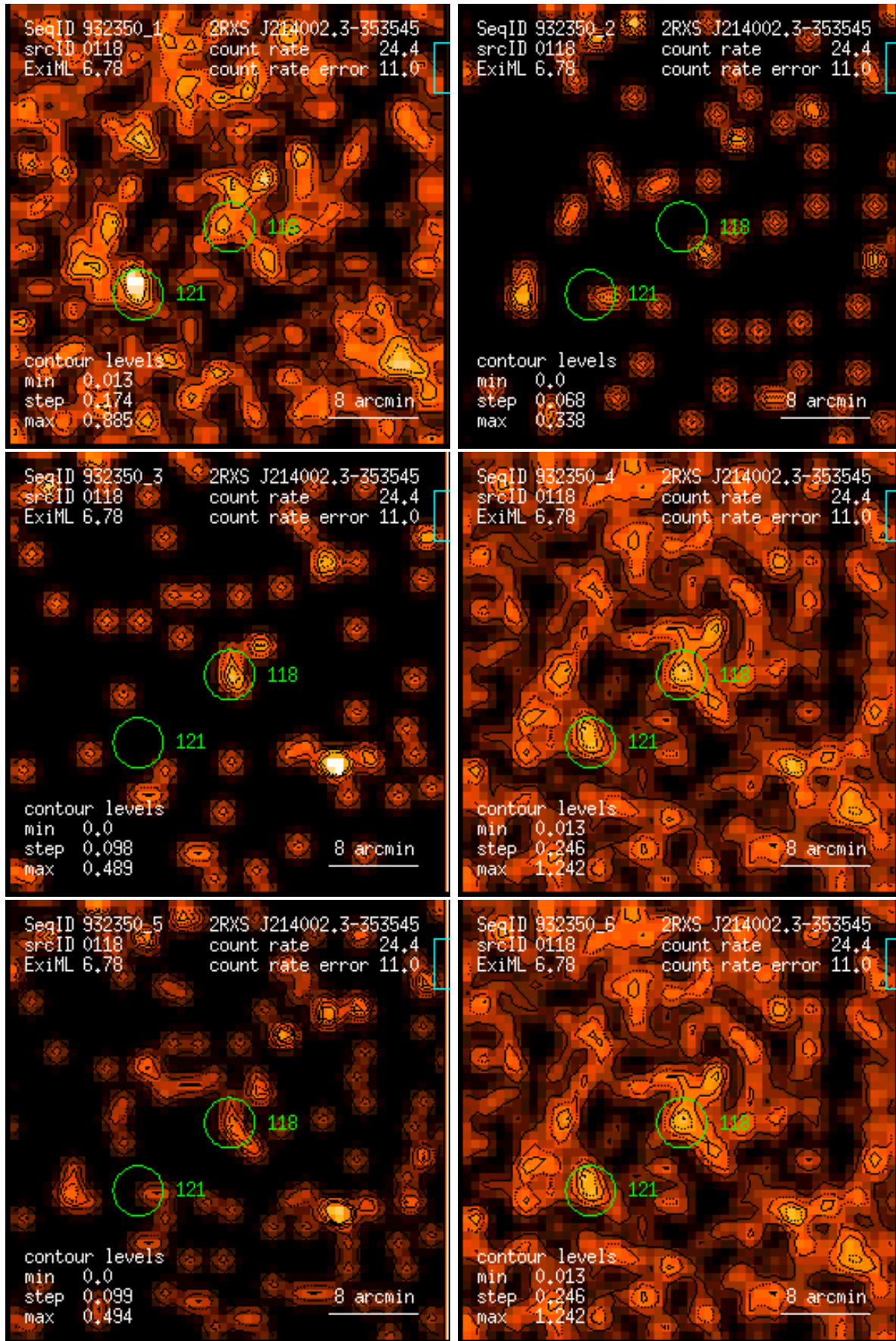
Figure 118: RASS 932350: detection 0118: band rate images, Gaussian filter: (1) PSPC channels 11 – 41, (2) 52 – 90, (3) 91 – 201, (4) 11 – 235, (5) 52 – 201, (6) 11 – 201. Broad band rates in counts/ks. Band rate contour levels in counts/ks/arcmin 2 .
