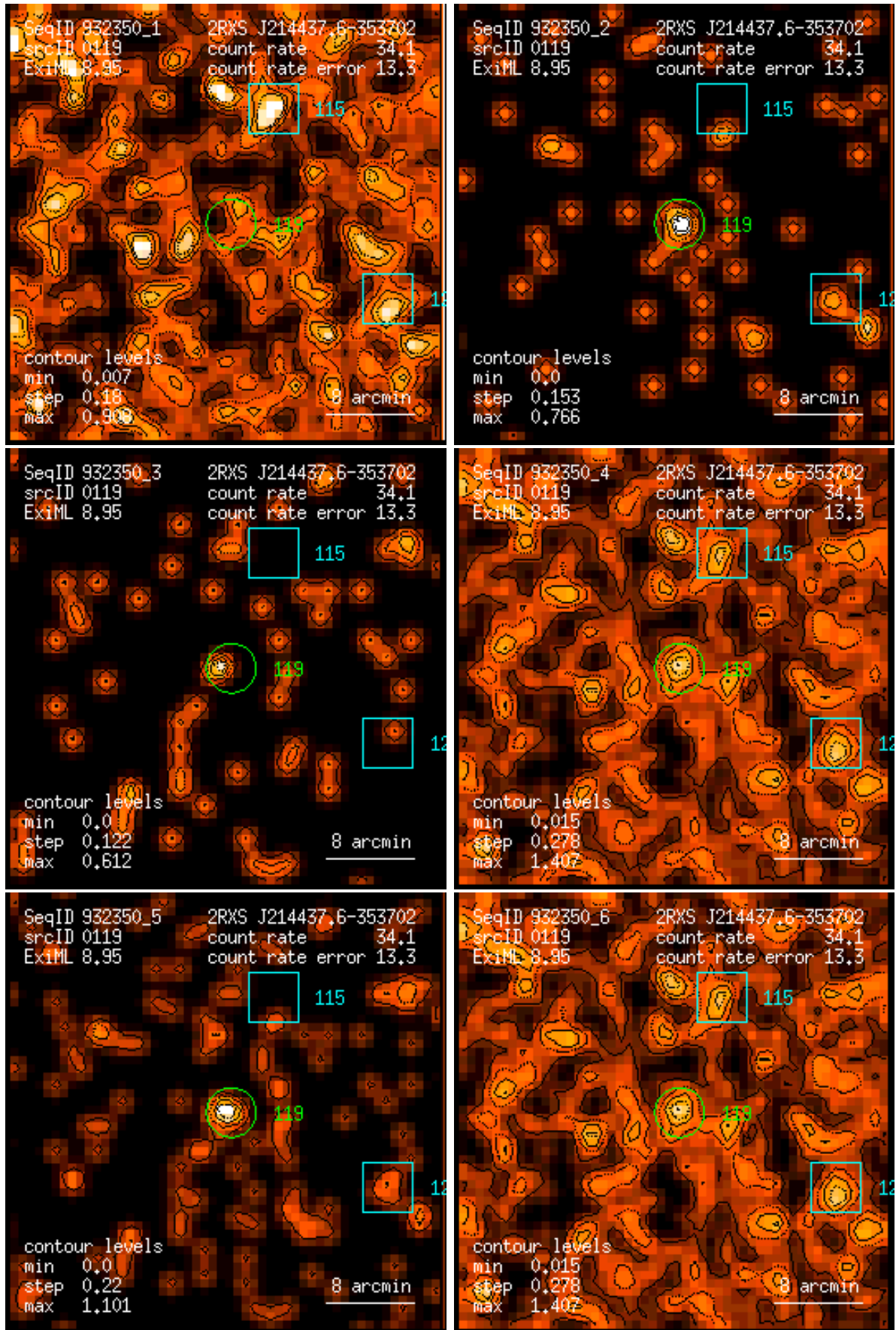
Figure 119: RASS 932350: detection 0119: band rate images, Gaussian filter: (1) PSPC channels 11 – 41, (2) 52 – 90, (3) 91 – 201, (4) 11 – 235, (5) 52 – 201, (6) 11 – 201. Broad band rates in counts/ks. Band rate contour levels in counts/ks/arcmin 2 .
