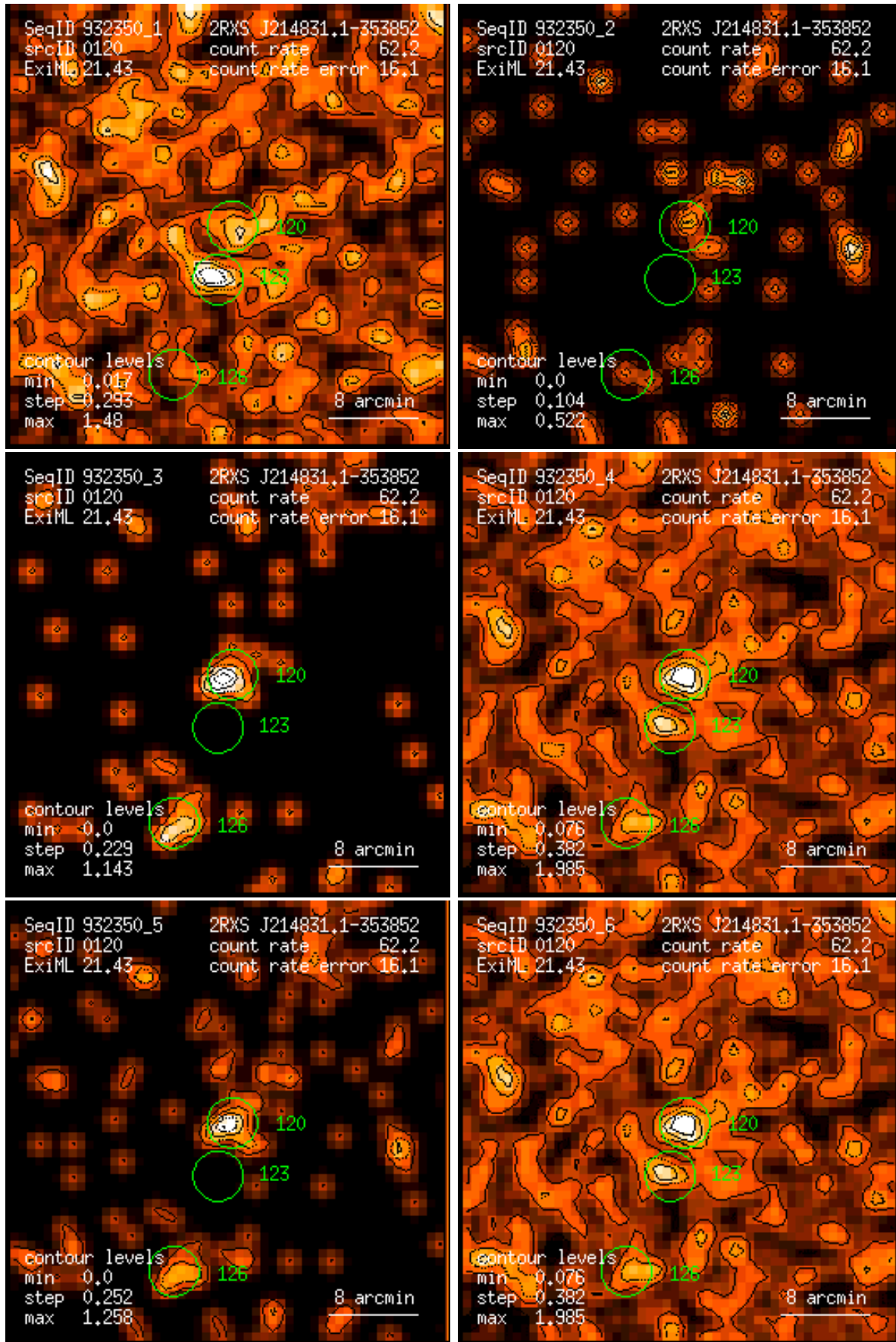
Figure 120: RASS 932350: detection 0120: band rate images, Gaussian filter: (1) PSPC channels 11 – 41, (2) 52 – 90, (3) 91 – 201, (4) 11 – 235, (5) 52 – 201, (6) 11 – 201. Broad band rates in counts/ks. Band rate contour levels in counts/ks/arcmin 2 .
