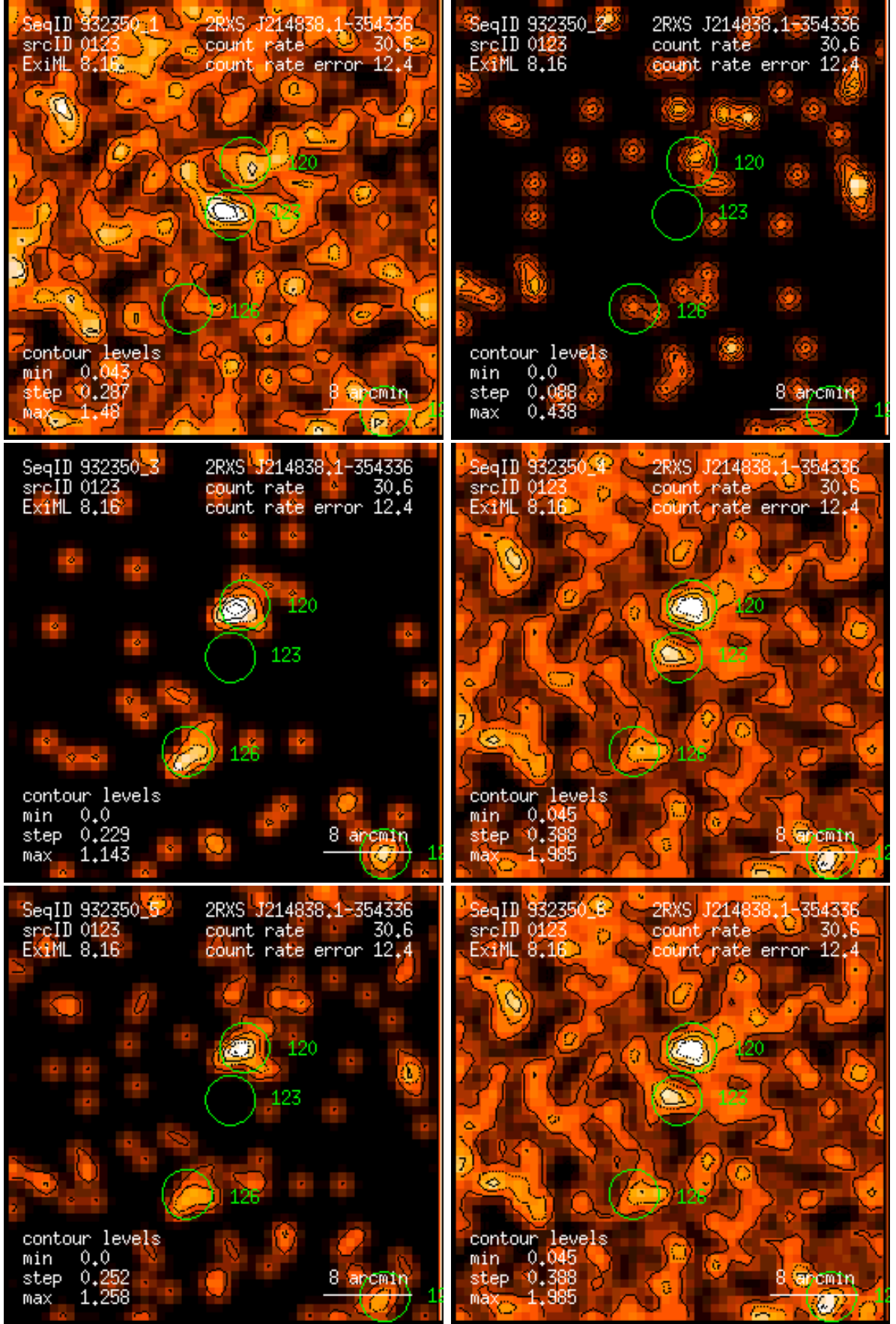
Figure 123: RASS 932350: detection 0123: band rate images, Gaussian filter: (1) PSPC channels 11 – 41, (2) 52 – 90, (3) 91 – 201, (4) 11 – 235, (5) 52 – 201, (6) 11 – 201. Broad band rates in counts/ks. Band rate contour levels in counts/ks/arcmin 2 .
