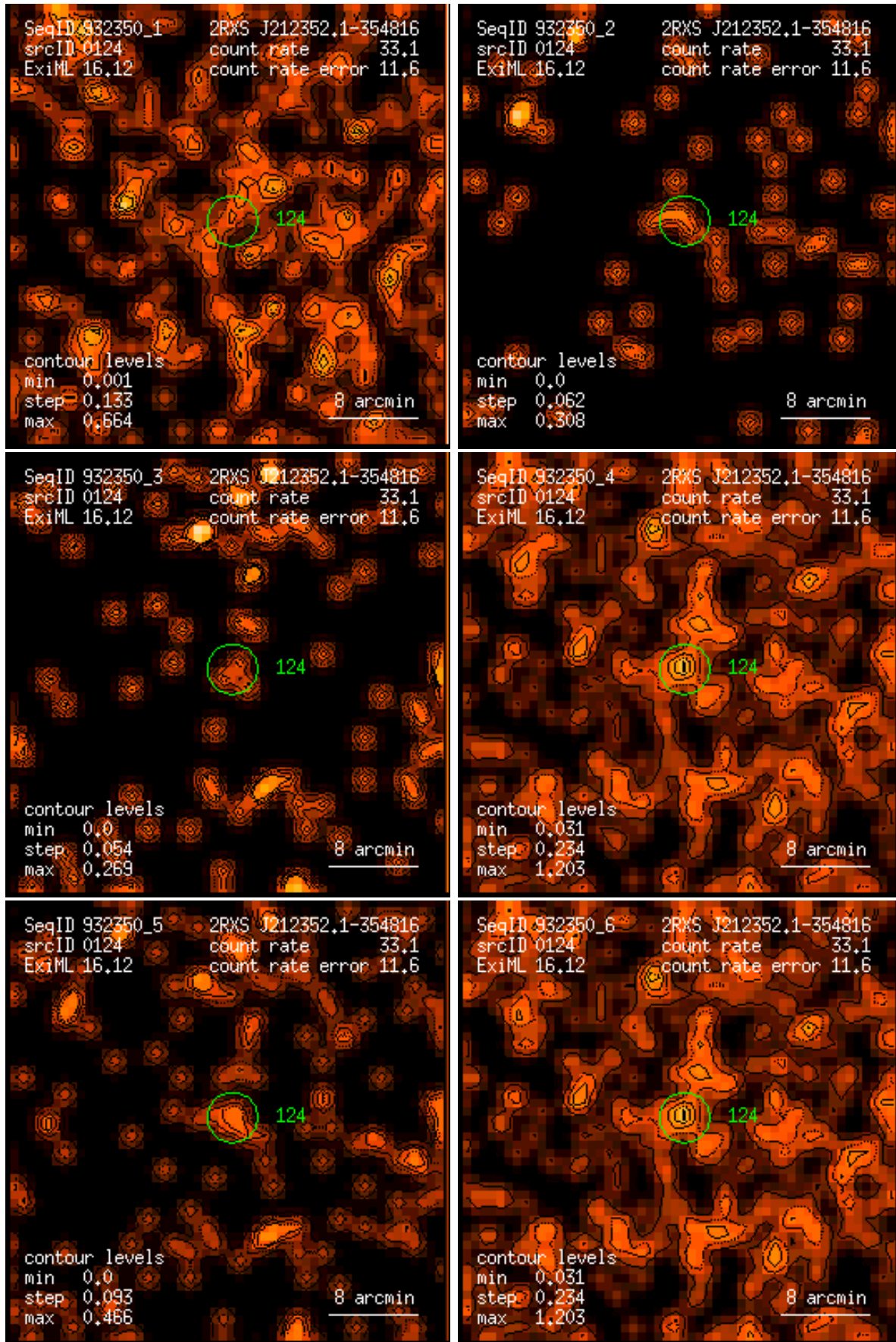
Figure 124: RASS 932350: detection 0124: band rate images, Gaussian filter: (1) PSPC channels 11 – 41, (2) 52 – 90, (3) 91 – 201, (4) 11 – 235, (5) 52 – 201, (6) 11 – 201. Broad band rates in counts/ks. Band rate contour levels in counts/ks/arcmin 2 .
