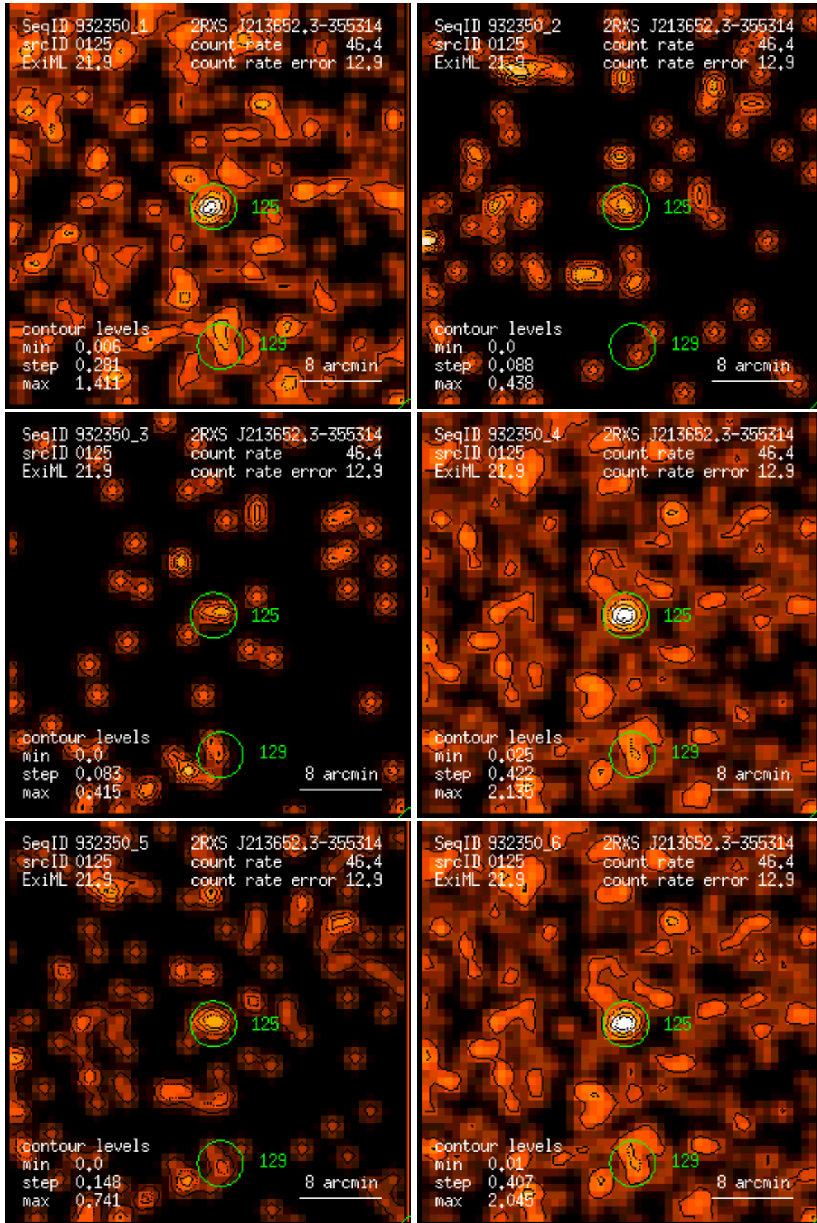
Figure 125: RASS 932350: detection 0125: band rate images, Gaussian filter: (1) PSPC channels 11 – 41, (2) 52 – 90, (3) 91 – 201, (4) 11 – 235, (5) 52 – 201, (6) 11 – 201. Broad band rates in counts/ks. Band rate contour levels in counts/ks/arcmin 2 .
