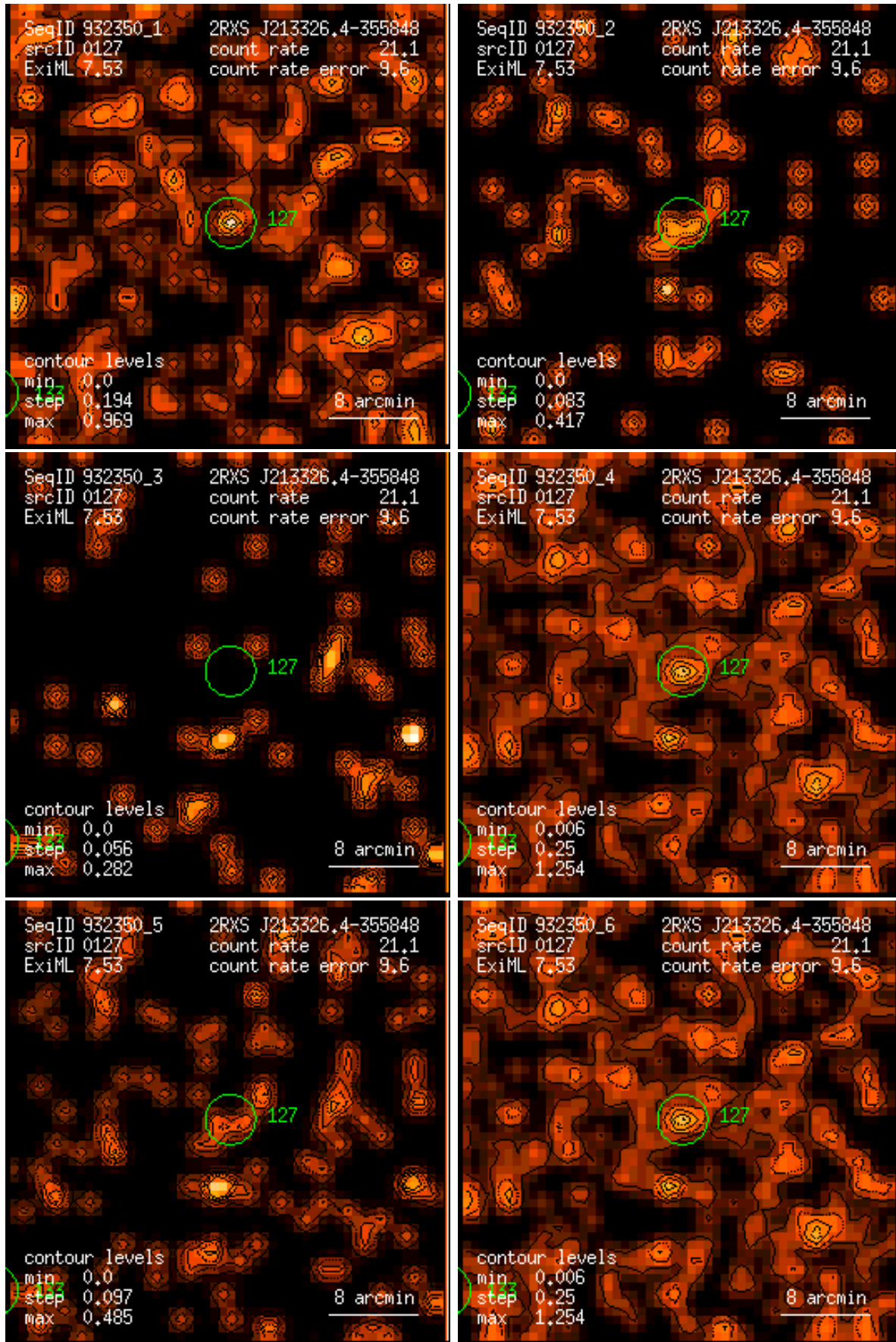
Figure 127: RASS 932350: detection 0127: band rate images, Gaussian filter: (1) PSPC channels 11 – 41, (2) 52 – 90, (3) 91 – 201, (4) 11 – 235, (5) 52 – 201, (6) 11 – 201. Broad band rates in counts/ks. Band rate contour levels in counts/ks/arcmin 2 .
