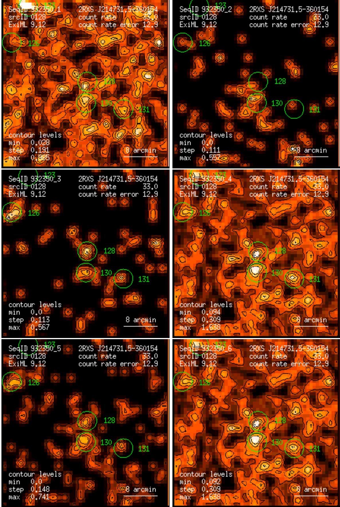
Figure 128: RASS 932350: detection 0128: band rate images, Gaussian filter: (1) PSPC channels 11 – 41, (2) 52 – 90, (3) 91 – 201, (4) 11 – 235, (5) 52 – 201, (6) 11 – 201. Broad band rates in counts/ks. Band rate contour levels in counts/ks/arcmin 2 .
