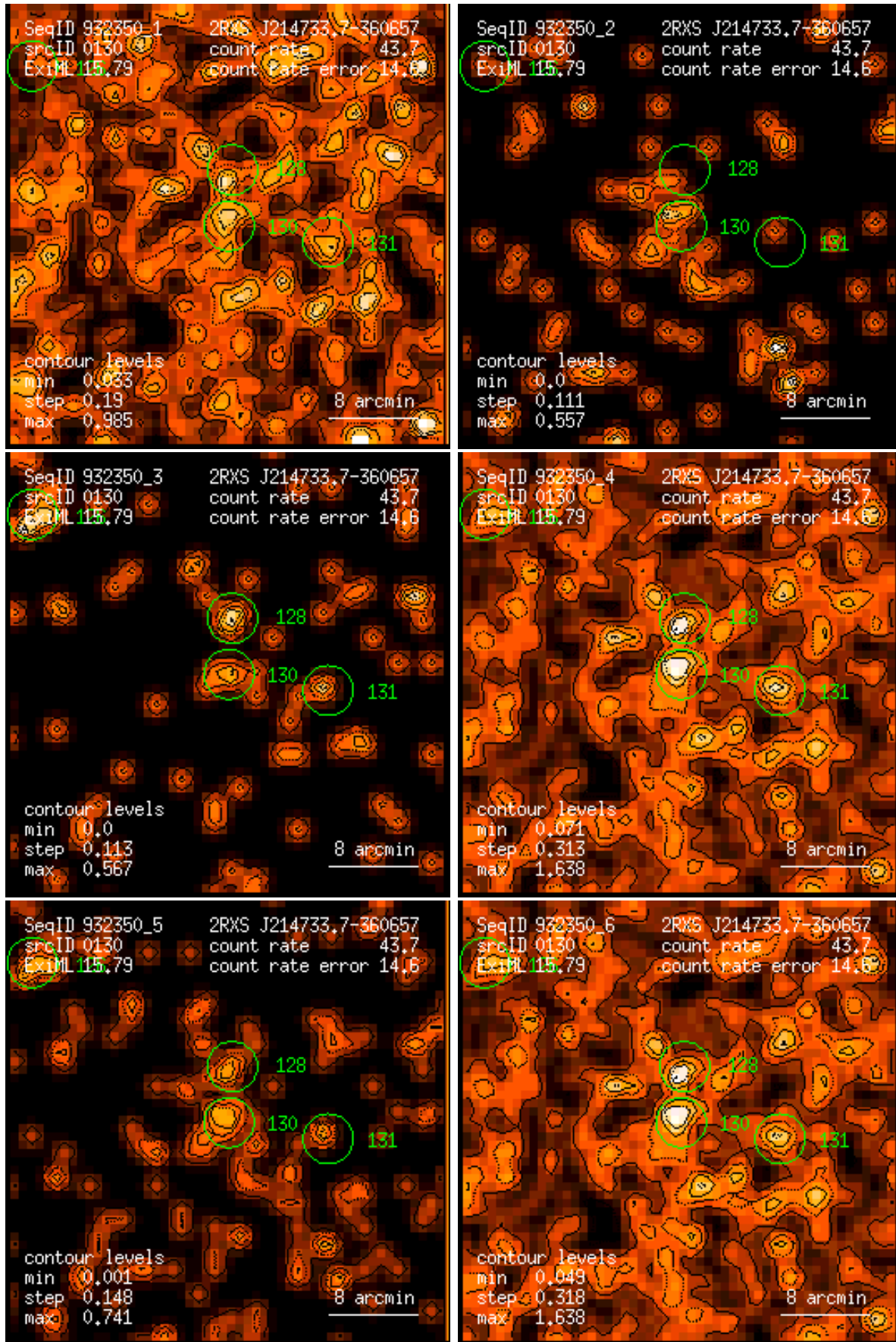
Figure 130: RASS 932350: detection 0130: band rate images, Gaussian filter: (1) PSPC channels 11 – 41, (2) 52 – 90, (3) 91 – 201, (4) 11 – 235, (5) 52 – 201, (6) 11 – 201. Broad band rates in counts/ks. Band rate contour levels in counts/ks/arcmin 2 .
