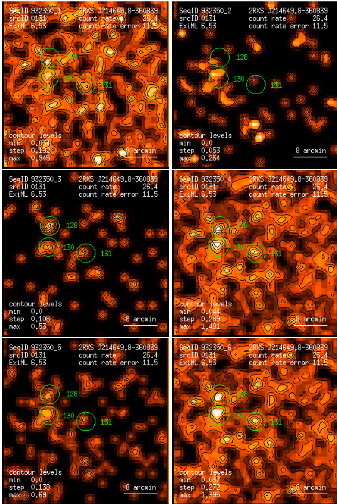
Figure 131: RASS 932350: detection 0131: band rate images, Gaussian filter: (1) PSPC channels 11 – 41, (2) 52 – 90, (3) 91 – 201, (4) 11 – 235, (5) 52 – 201, (6) 11 – 201. Broad band rates in counts/ks. Band rate contour levels in counts/ks/arcmin 2 .
