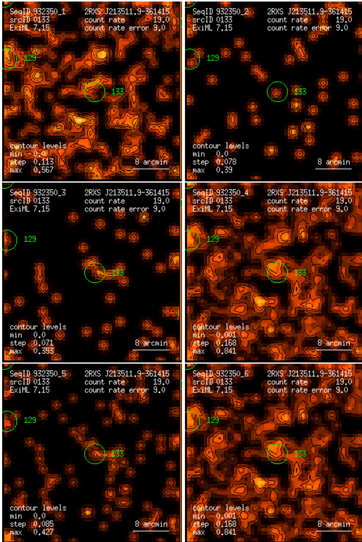
Figure 133: RASS 932350: detection 0133: band rate images, Gaussian filter: (1) PSPC channels 11 – 41, (2) 52 – 90, (3) 91 – 201, (4) 11 – 235, (5) 52 – 201, (6) 11 – 201. Broad band rates in counts/ks. Band rate contour levels in counts/ks/arcmin 2 .
