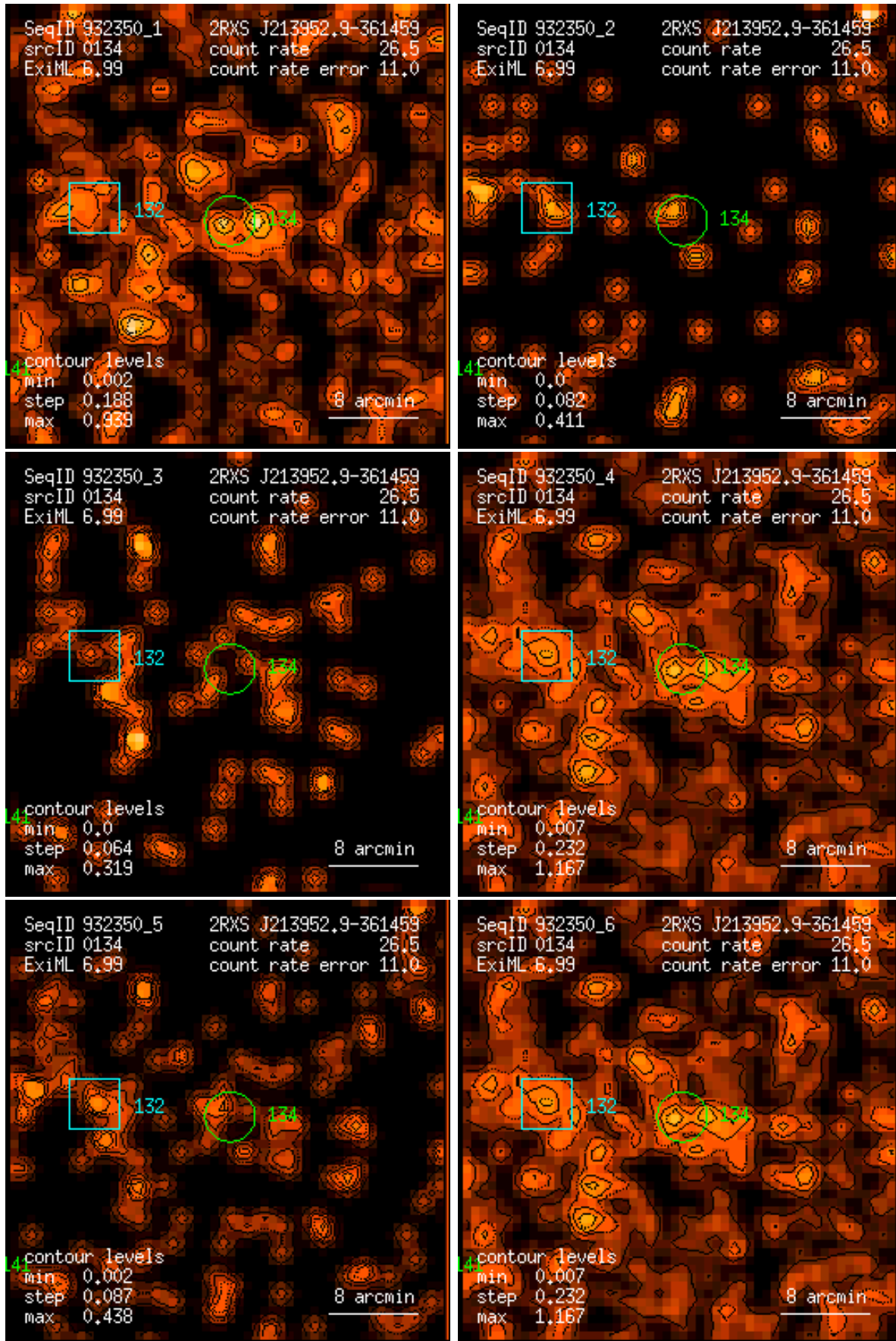
Figure 134: RASS 932350: detection 0134: band rate images, Gaussian filter: (1) PSPC channels 11 – 41, (2) 52 – 90, (3) 91 – 201, (4) 11 – 235, (5) 52 – 201, (6) 11 – 201. Broad band rates in counts/ks. Band rate contour levels in counts/ks/arcmin 2 .
