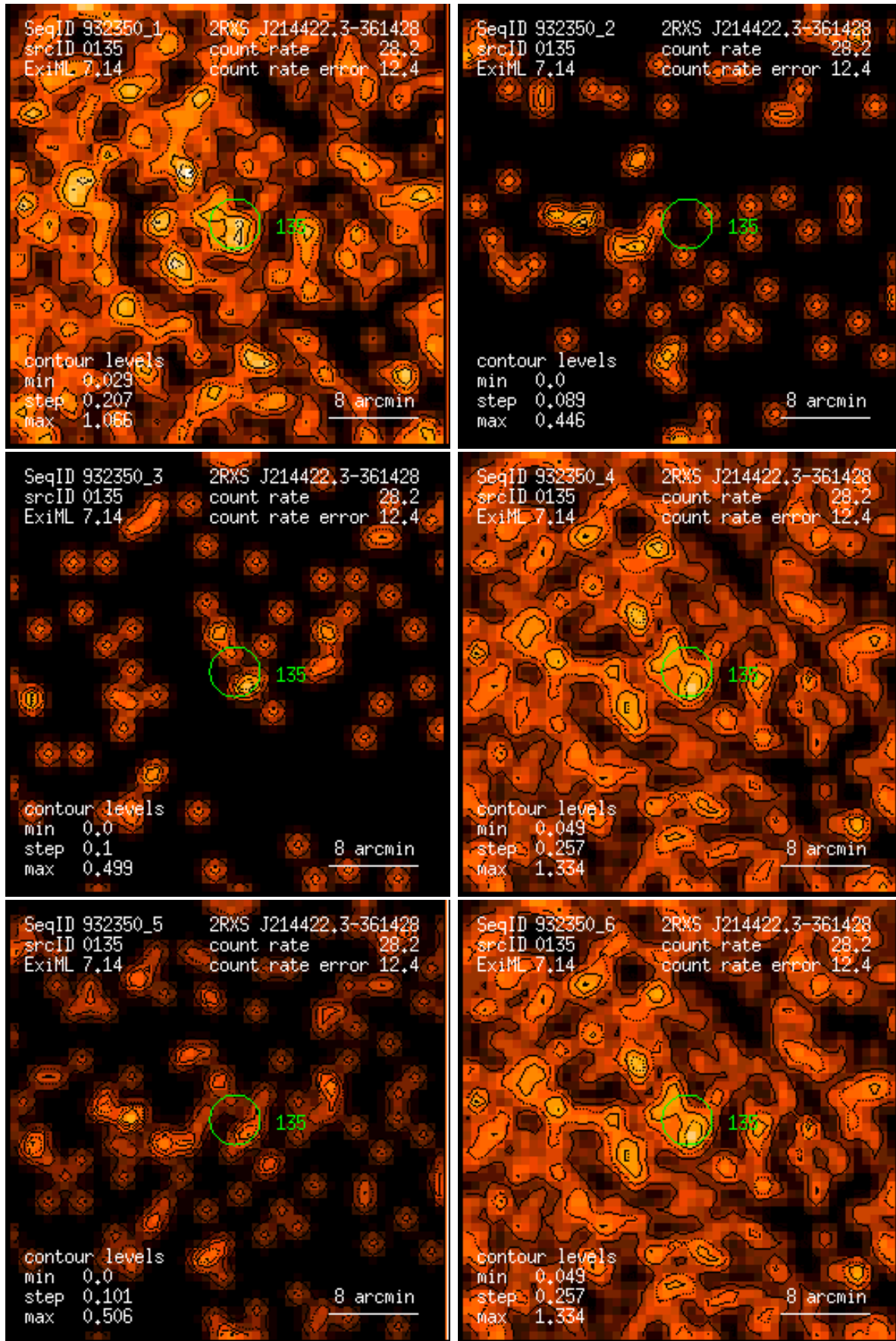
Figure 135: RASS 932350: detection 0135: band rate images, Gaussian filter: (1) PSPC channels 11 – 41, (2) 52 – 90, (3) 91 – 201, (4) 11 – 235, (5) 52 – 201, (6) 11 – 201. Broad band rates in counts/ks. Band rate contour levels in counts/ks/arcmin 2 .
