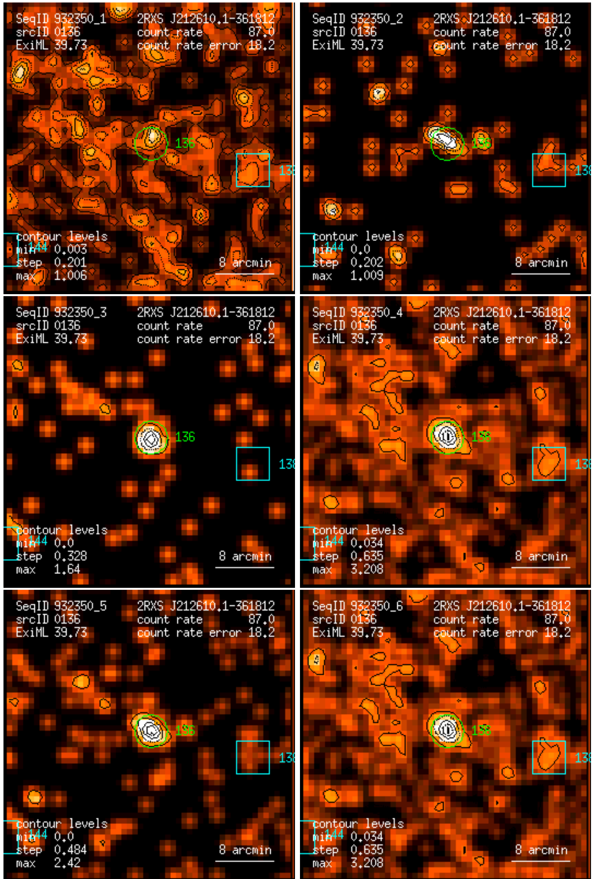
Figure 136: RASS 932350: detection 0136: band rate images, Gaussian filter: (1) PSPC channels 11 – 41, (2) 52 – 90, (3) 91 – 201, (4) 11 – 235, (5) 52 – 201, (6) 11 – 201. Broad band rates in counts/ks. Band rate contour levels in counts/ks/arcmin 2 .
