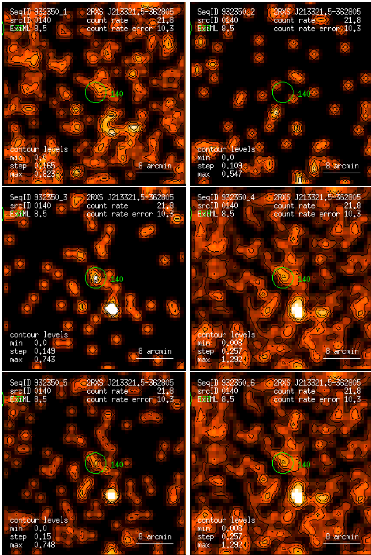
Figure 140: RASS 932350: detection 0140: band rate images, Gaussian filter: (1) PSPC channels 11 – 41, (2) 52 – 90, (3) 91 – 201, (4) 11 – 235, (5) 52 – 201, (6) 11 – 201. Broad band rates in counts/ks. Band rate contour levels in counts/ks/arcmin 2 .
