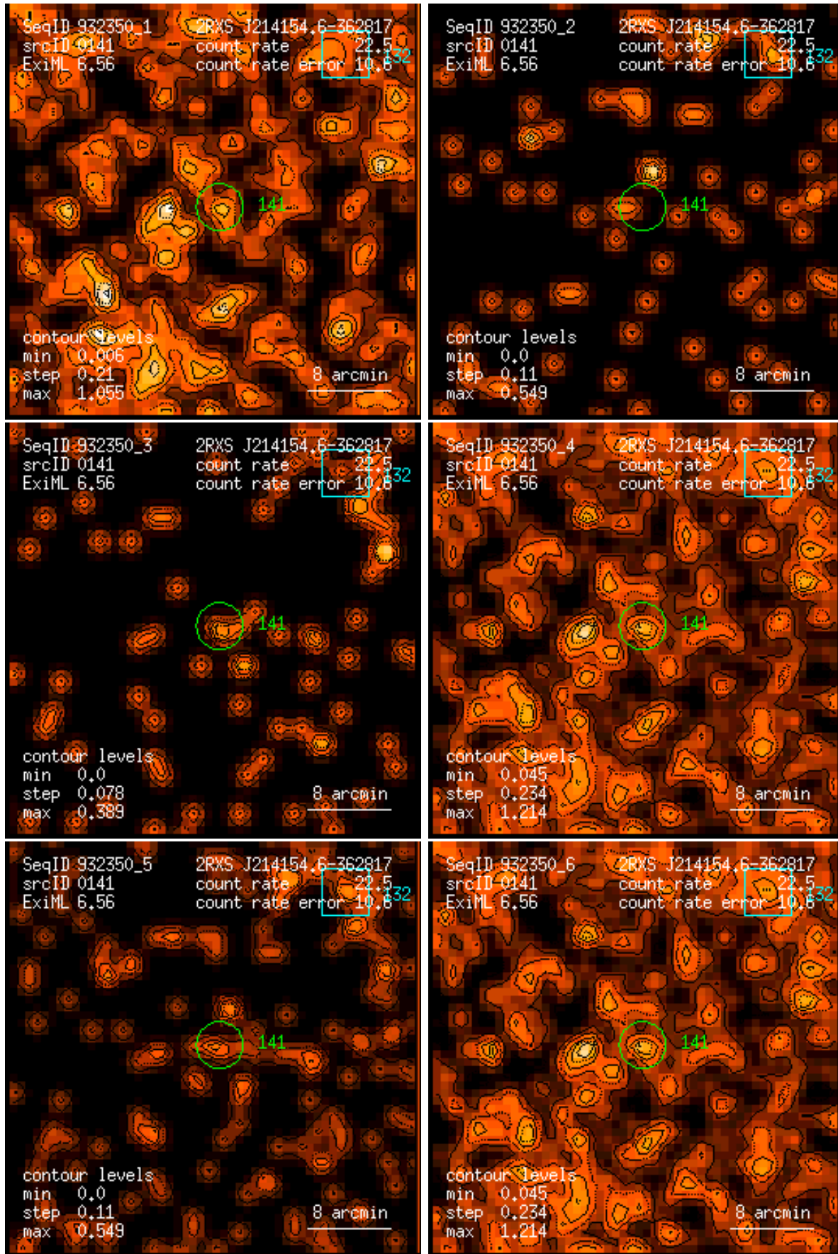
Figure 141: RASS 932350: detection 0141: band rate images, Gaussian filter: (1) PSPC channels 11 – 41, (2) 52 – 90, (3) 91 – 201, (4) 11 – 235, (5) 52 – 201, (6) 11 – 201. Broad band rates in counts/ks. Band rate contour levels in counts/ks/arcmin 2 .
