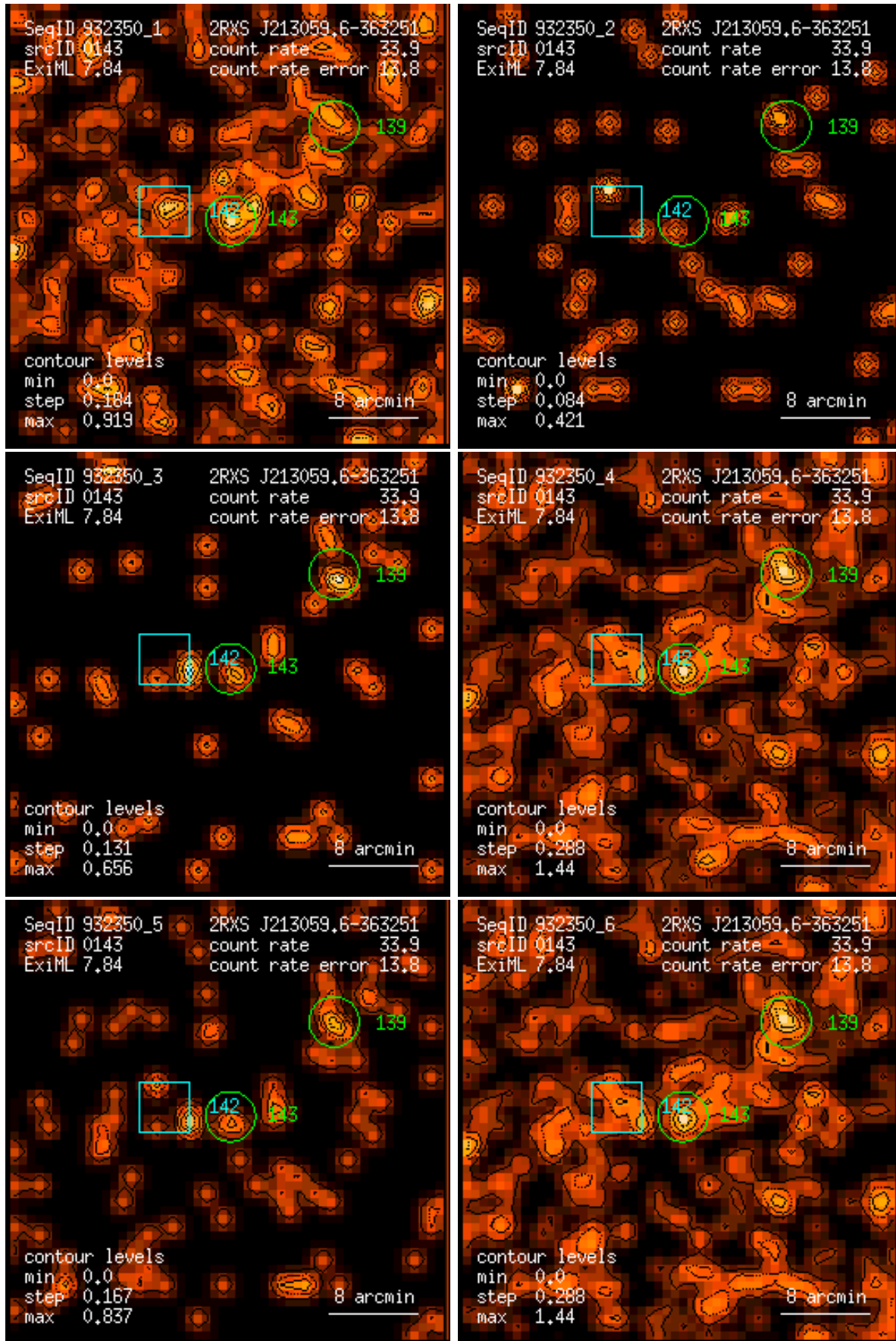
Figure 143: RASS 932350: detection 0143: band rate images, Gaussian filter: (1) PSPC channels 11 – 41, (2) 52 – 90, (3) 91 – 201, (4) 11 – 235, (5) 52 – 201, (6) 11 – 201. Broad band rates in counts/ks. Band rate contour levels in counts/ks/arcmin 2 .
