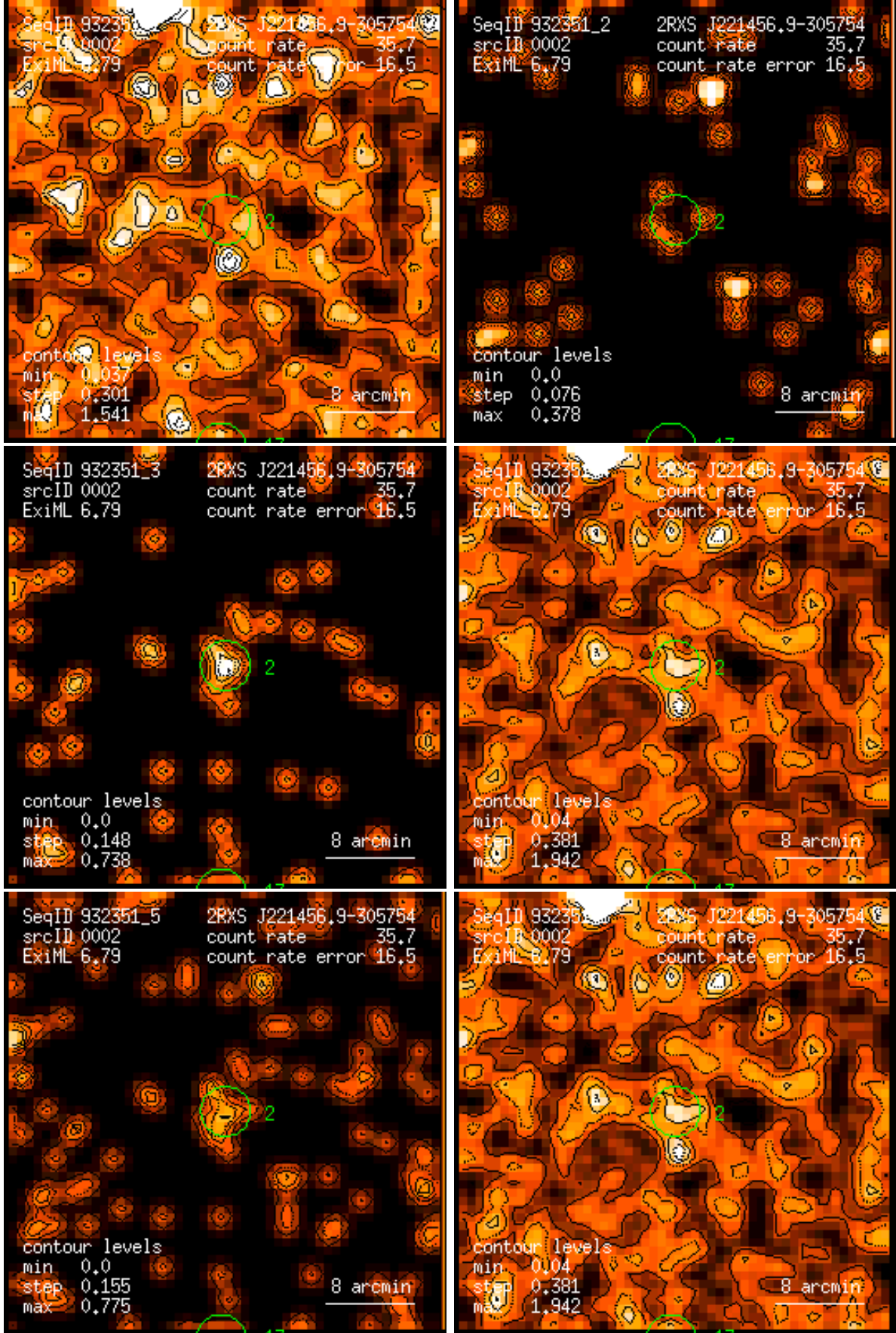
Figure 2: RASS 932351: detection 0002: band rate images, Gaussian filter: (1) PSPC channels 11 – 41, (2) 52 – 90, (3) 91 – 201, (4) 11 – 235, (5) 52 – 201, (6) 11 – 201. Broad band rates in counts/ks. Band rate contour levels in counts/ks/arcmin 2 .
