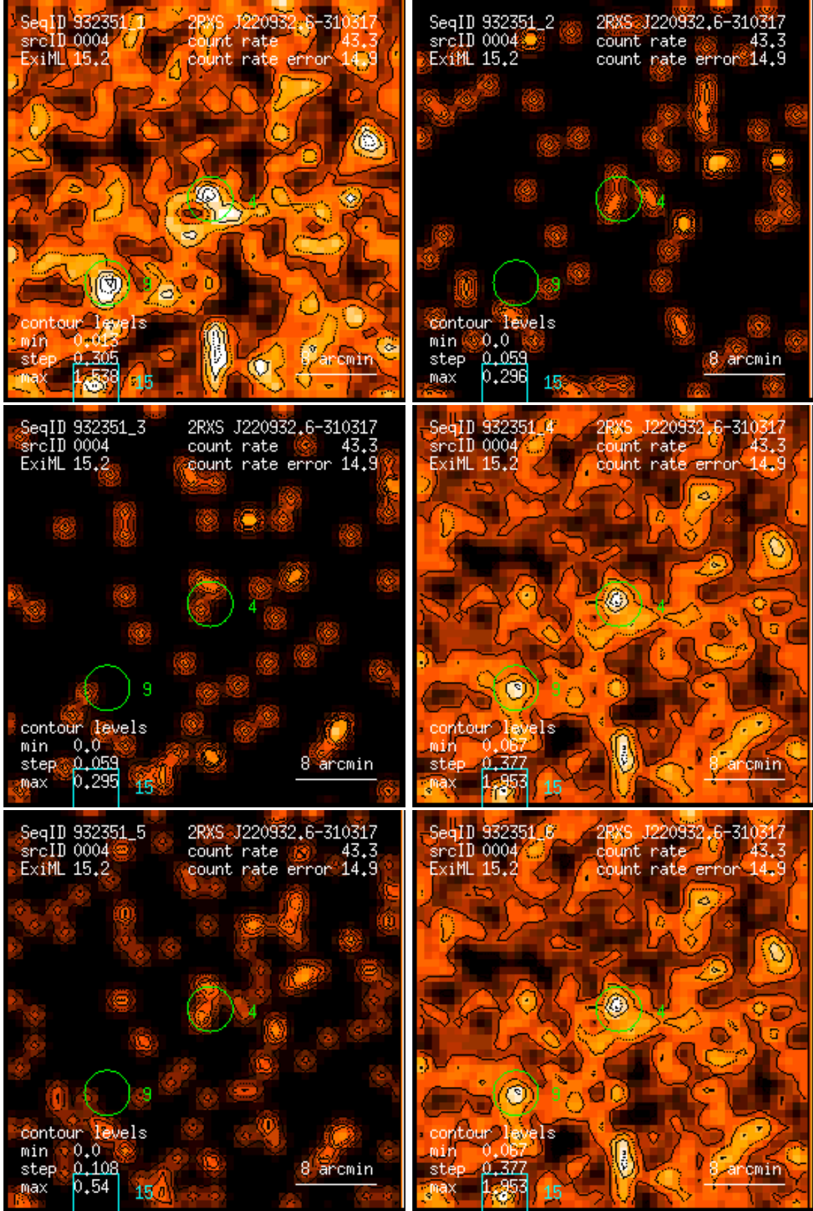
Figure 4: RASS 932351: detection 0004: band rate images, Gaussian filter: (1) PSPC channels 11 – 41, (2) 52 – 90, (3) 91 – 201, (4) 11 – 235, (5) 52 – 201, (6) 11 – 201. Broad band rates in counts/ks. Band rate contour levels in counts/ks/arcmin 2 .
