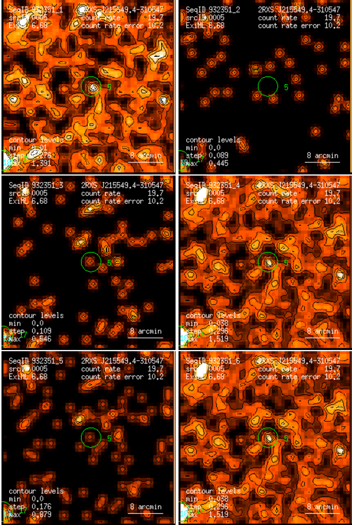
Figure 5: RASS 932351: detection 0005: band rate images, Gaussian filter: (1) PSPC channels 11 – 41, (2) 52 – 90, (3) 91 – 201, (4) 11 – 235, (5) 52 – 201, (6) 11 – 201. Broad band rates in counts/ks. Band rate contour levels in counts/ks/arcmin 2 .
