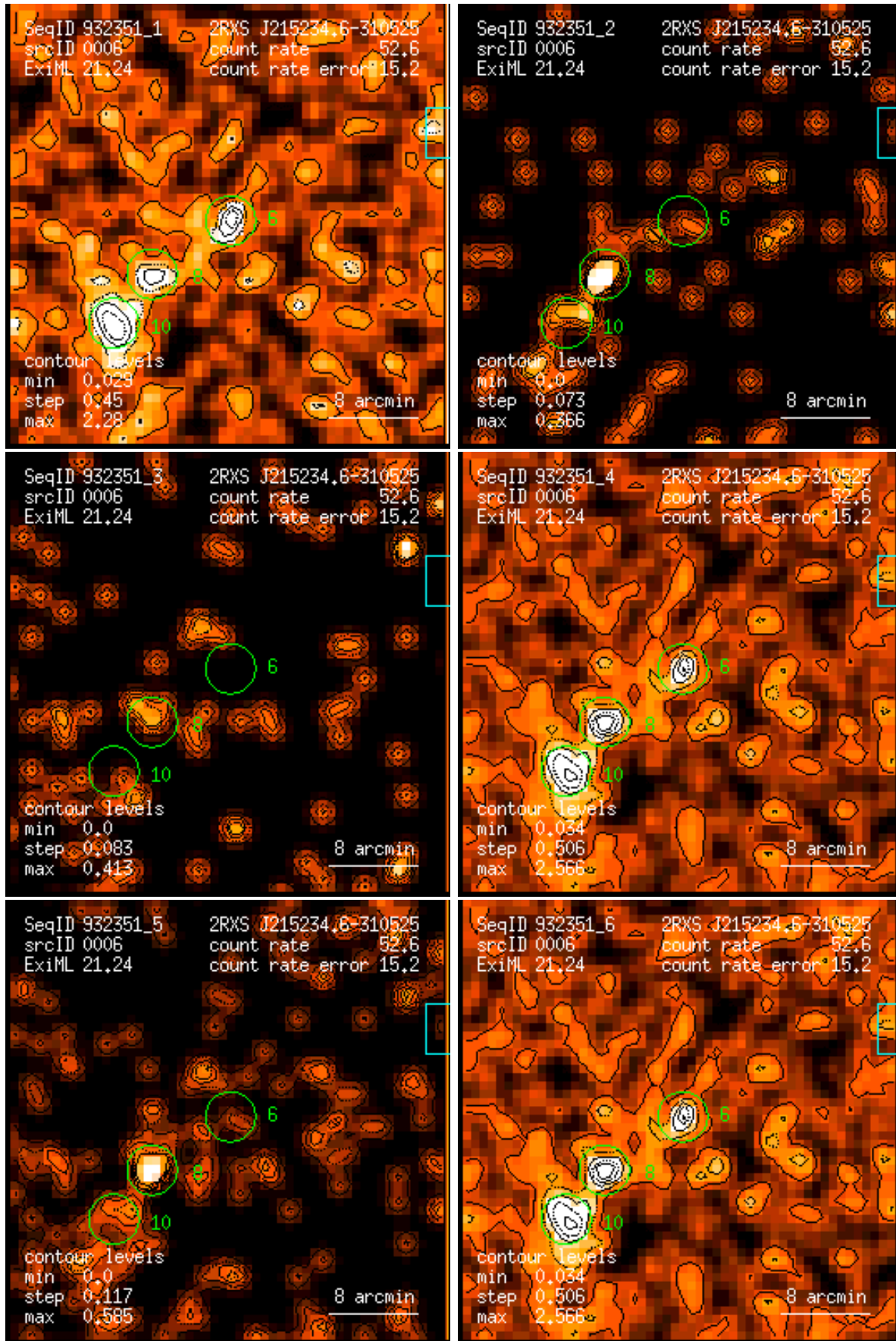
Figure 6: RASS 932351: detection 0006: band rate images, Gaussian filter: (1) PSPC channels 11 – 41, (2) 52 – 90, (3) 91 – 201, (4) 11 – 235, (5) 52 – 201, (6) 11 – 201. Broad band rates in counts/ks. Band rate contour levels in counts/ks/arcmin 2 .
