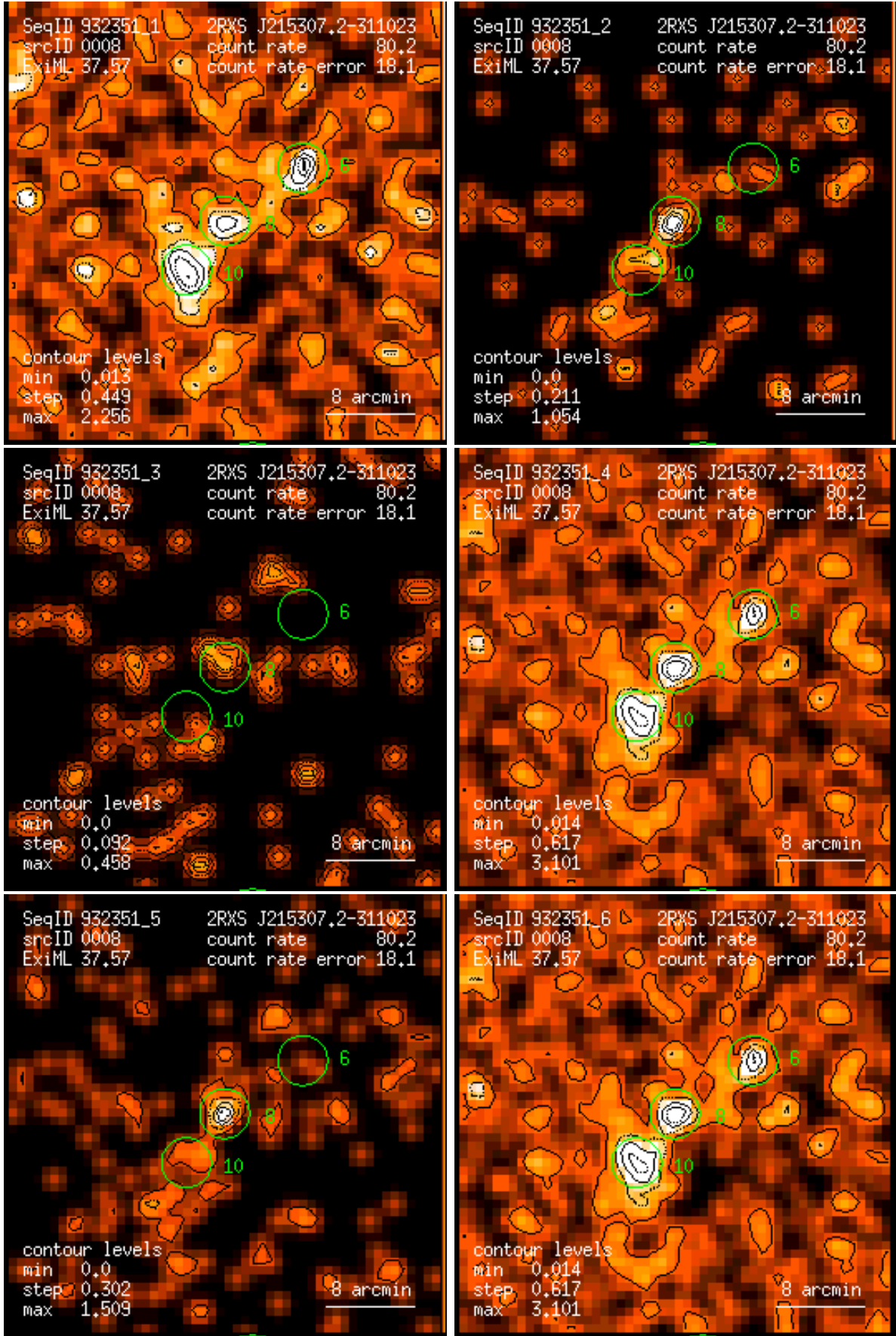
Figure 8: RASS 932351: detection 0008: band rate images, Gaussian filter: (1) PSPC channels 11 – 41, (2) 52 – 90, (3) 91 – 201, (4) 11 – 235, (5) 52 – 201, (6) 11 – 201. Broad band rates in counts/ks. Band rate contour levels in counts/ks/arcmin 2 .
