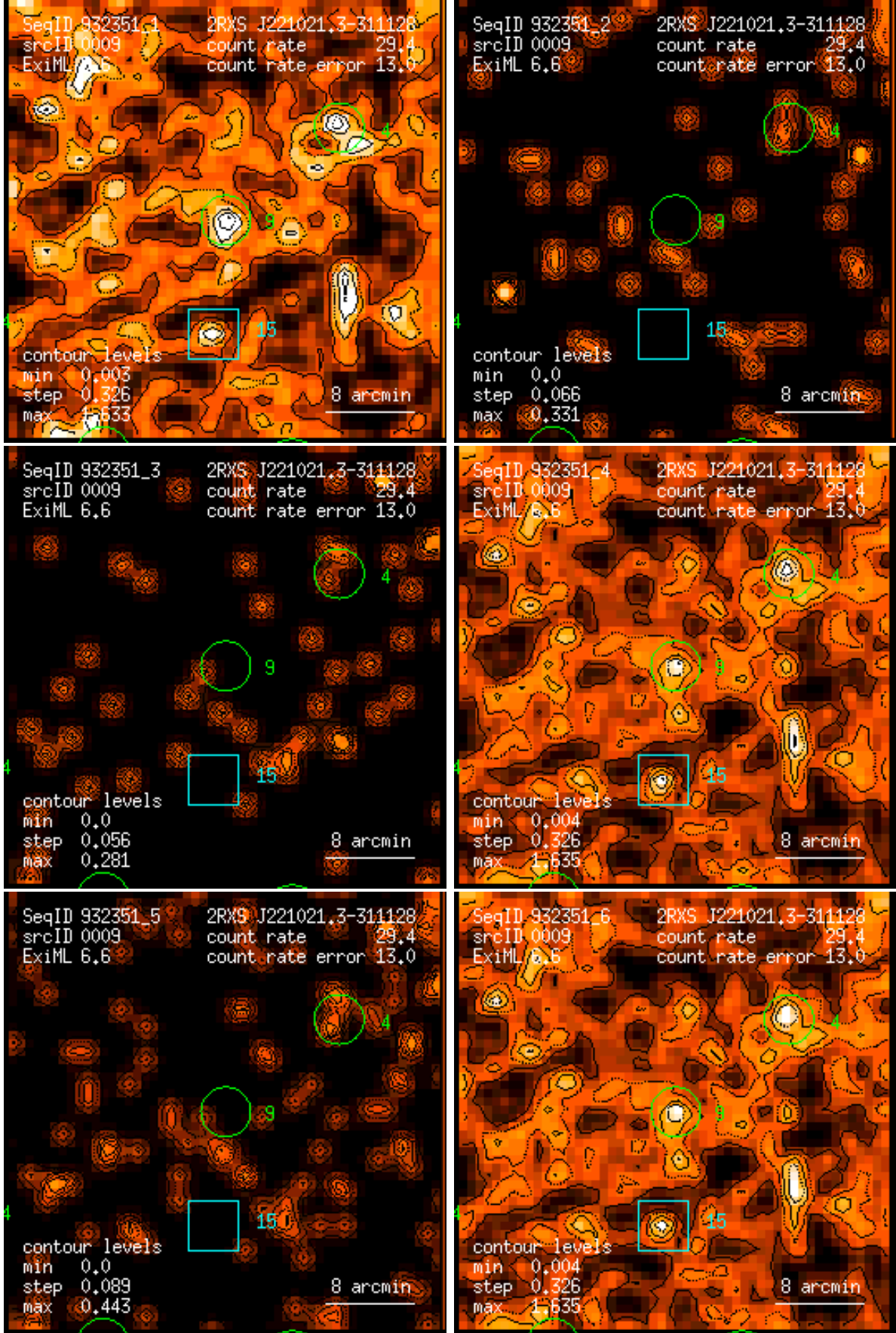
Figure 9: RASS 932351: detection 0009: band rate images, Gaussian filter: (1) PSPC channels 11 – 41, (2) 52 – 90, (3) 91 – 201, (4) 11 – 235, (5) 52 – 201, (6) 11 – 201. Broad band rates in counts/ks. Band rate contour levels in counts/ks/arcmin 2 .
