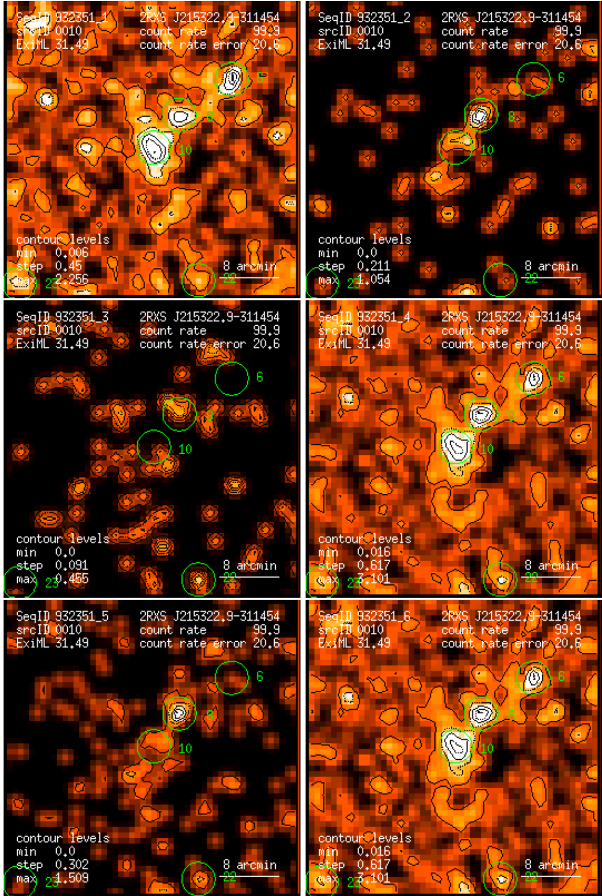
Figure 10: RASS 932351: detection 0010: band rate images, Gaussian filter: (1) PSPC channels 11 – 41, (2) 52 – 90, (3) 91 – 201, (4) 11 – 235, (5) 52 – 201, (6) 11 – 201. Broad band rates in counts/ks. Band rate contour levels in counts/ks/arcmin 2 .
