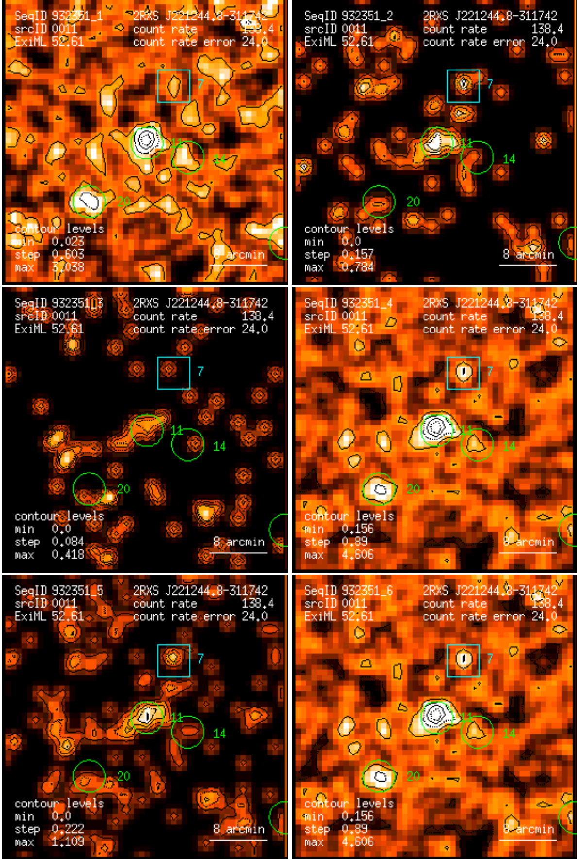
Figure 11: RASS 932351: detection 0011: band rate images, Gaussian filter: (1) PSPC channels 11 – 41, (2) 52 – 90, (3) 91 – 201, (4) 11 – 235, (5) 52 – 201, (6) 11 – 201. Broad band rates in counts/ks. Band rate contour levels in counts/ks/arcmin 2 .
