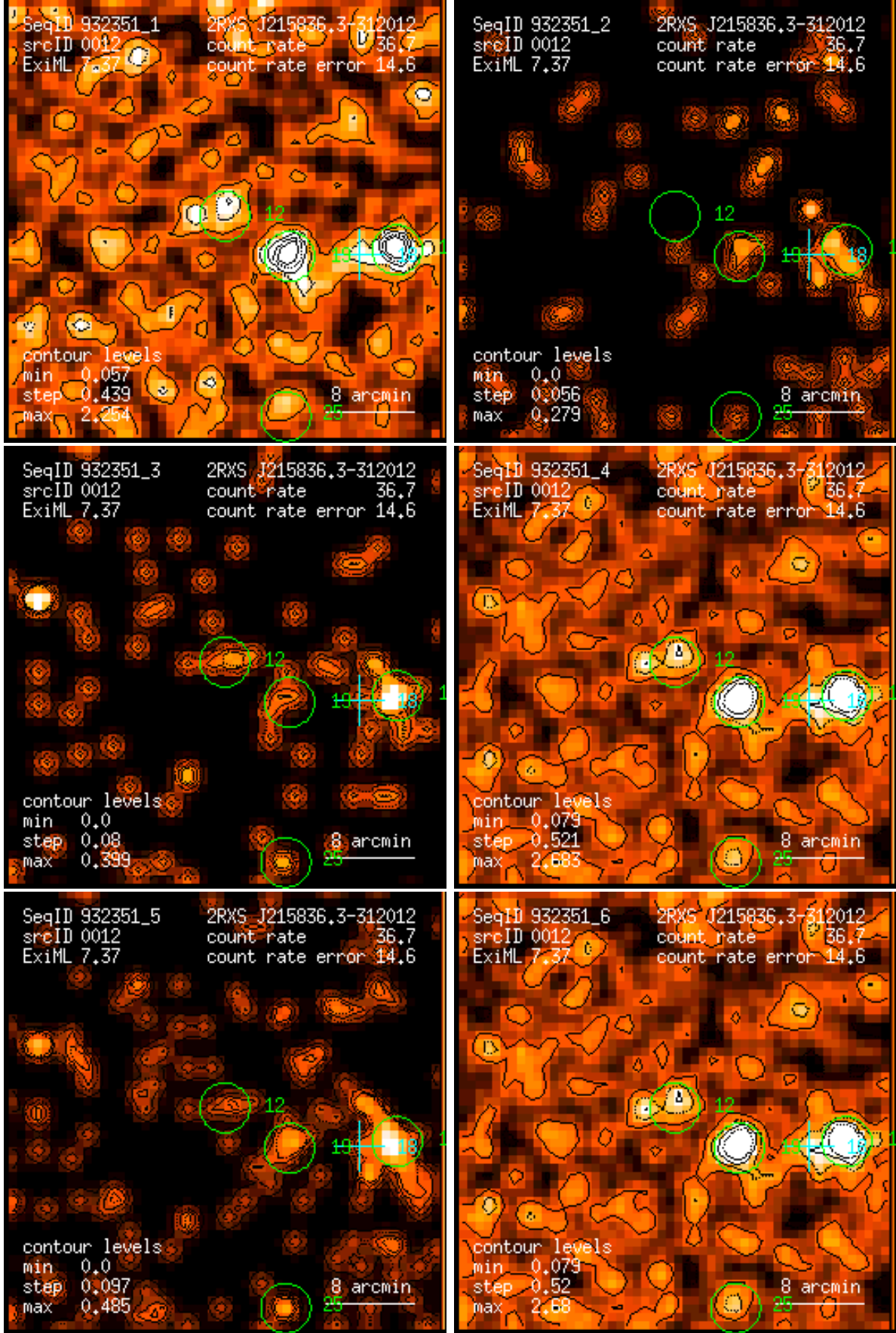
Figure 12: RASS 932351: detection 0012: band rate images, Gaussian filter: (1) PSPC channels 11 – 41, (2) 52 – 90, (3) 91 – 201, (4) 11 – 235, (5) 52 – 201, (6) 11 – 201. Broad band rates in counts/ks. Band rate contour levels in counts/ks/arcmin 2 .
