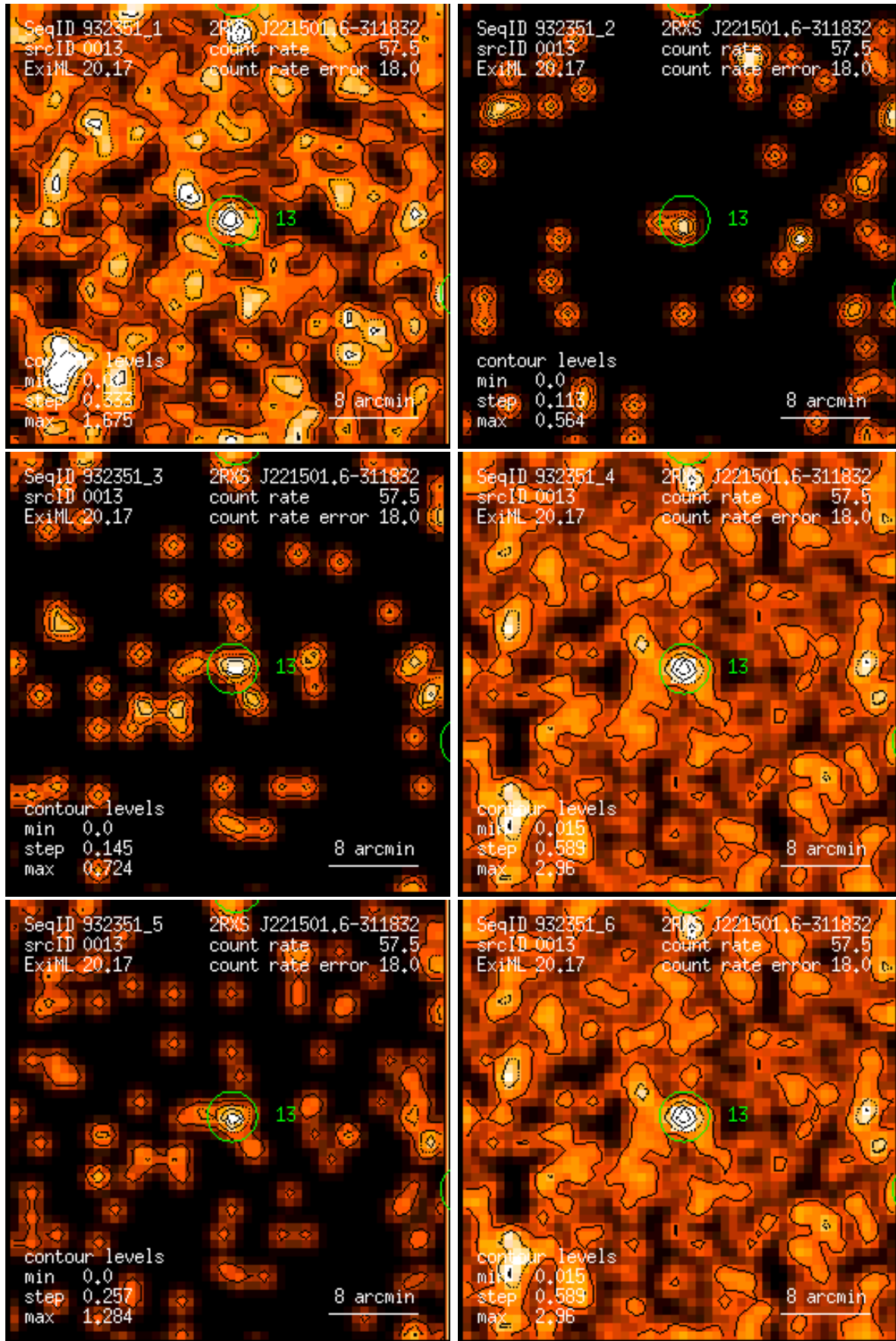
Figure 13: RASS 932351: detection 0013: band rate images, Gaussian filter: (1) PSPC channels 11 – 41, (2) 52 – 90, (3) 91 – 201, (4) 11 – 235, (5) 52 – 201, (6) 11 – 201. Broad band rates in counts/ks. Band rate contour levels in counts/ks/arcmin 2 .
