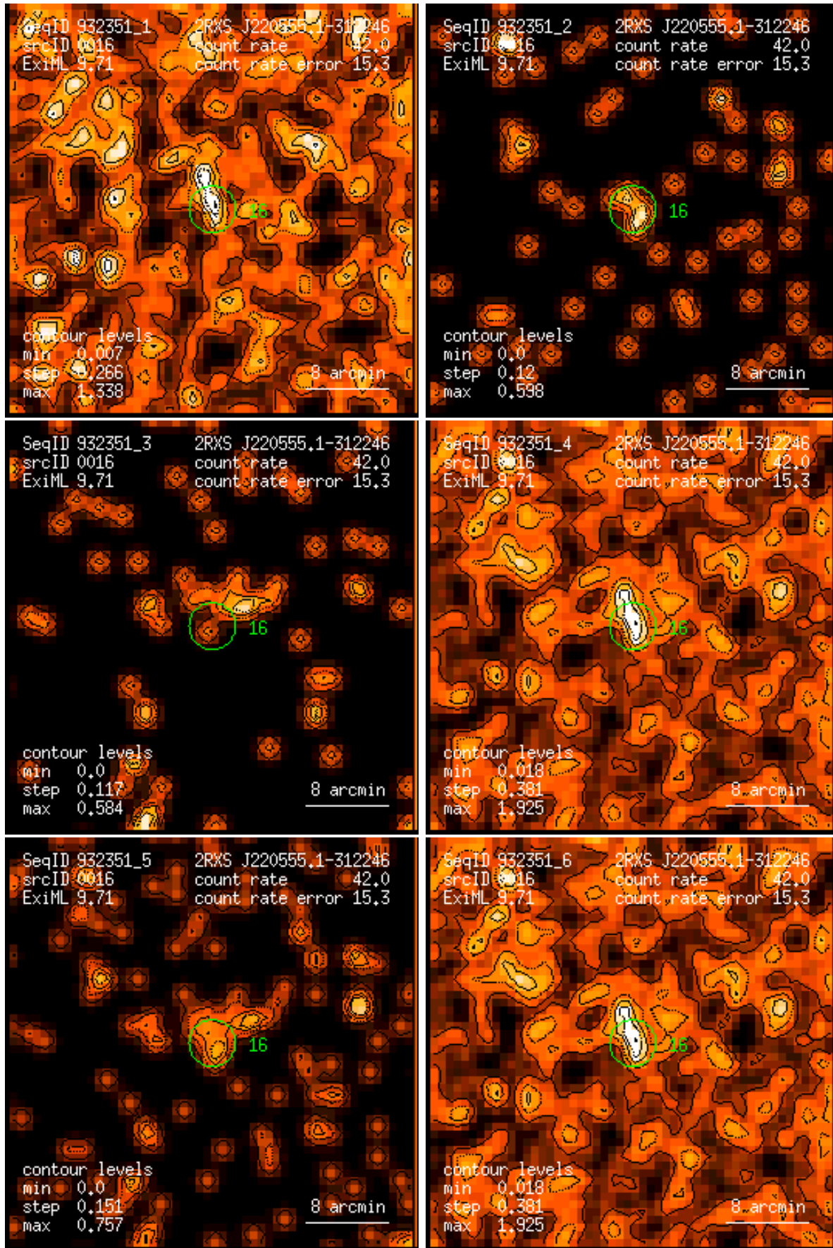
Figure 16: RASS 932351: detection 0016: band rate images, Gaussian filter: (1) PSPC channels 11 – 41, (2) 52 – 90, (3) 91 – 201, (4) 11 – 235, (5) 52 – 201, (6) 11 – 201. Broad band rates in counts/ks. Band rate contour levels in counts/ks/arcmin 2 .
