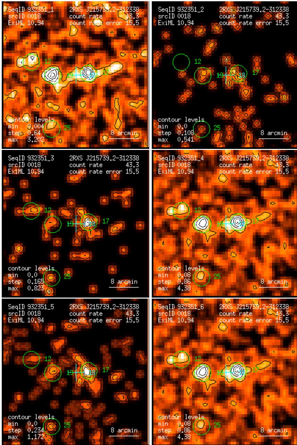
Figure 18: RASS 932351: detection 0018: band rate images, Gaussian filter: (1) PSPC channels 11 – 41, (2) 52 – 90, (3) 91 – 201, (4) 11 – 235, (5) 52 – 201, (6) 11 – 201. Broad band rates in counts/ks. Band rate contour levels in counts/ks/arcmin 2 .
