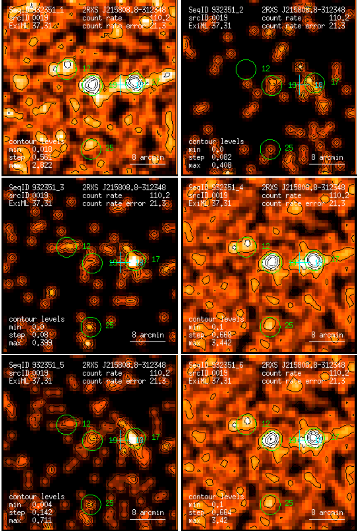
Figure 19: RASS 932351: detection 0019: band rate images, Gaussian filter: (1) PSPC channels 11 – 41, (2) 52 – 90, (3) 91 – 201, (4) 11 – 235, (5) 52 – 201, (6) 11 – 201. Broad band rates in counts/ks. Band rate contour levels in counts/ks/arcmin 2 .
