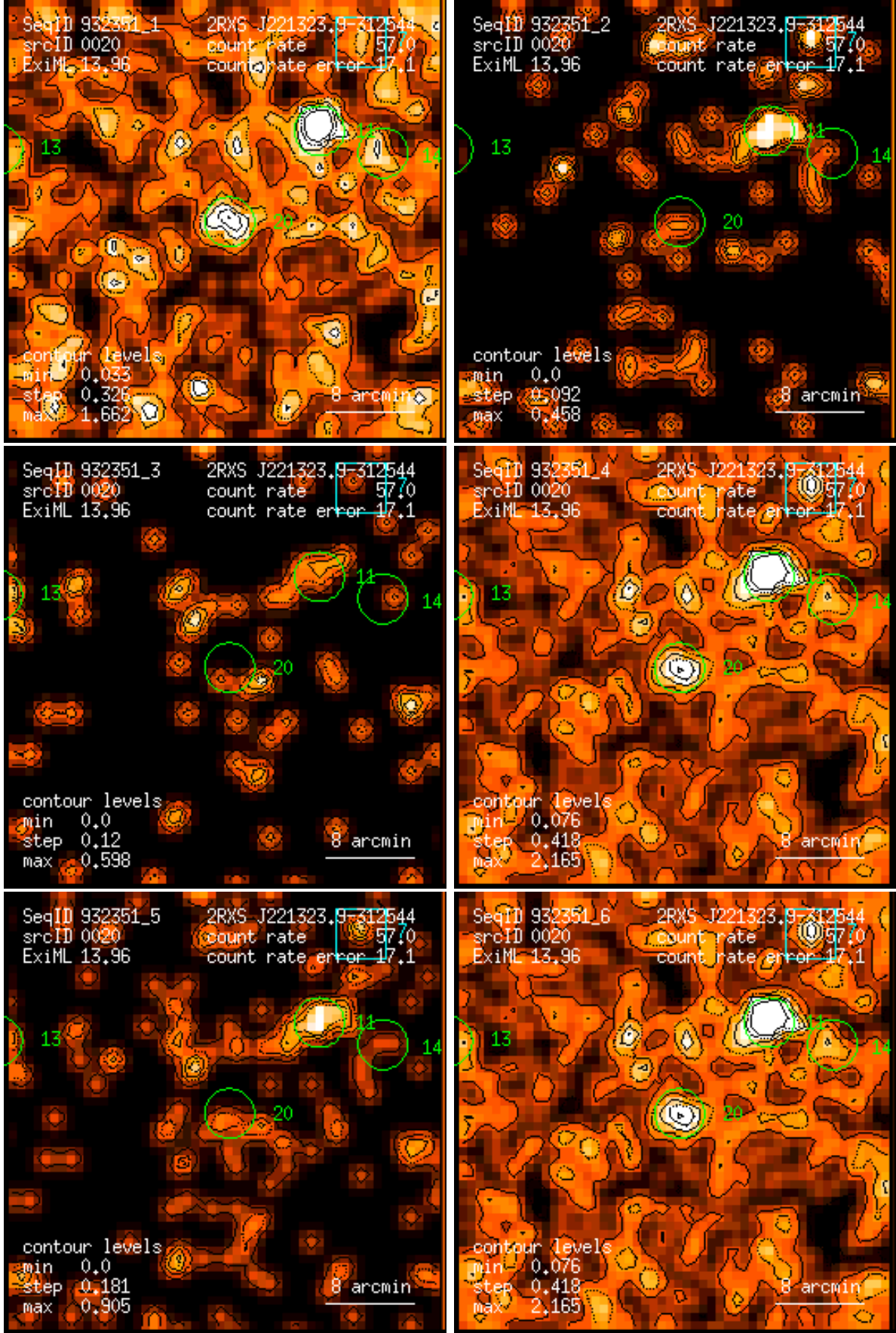
Figure 20: RASS 932351: detection 0020: band rate images, Gaussian filter: (1) PSPC channels 11 – 41, (2) 52 – 90, (3) 91 – 201, (4) 11 – 235, (5) 52 – 201, (6) 11 – 201. Broad band rates in counts/ks. Band rate contour levels in counts/ks/arcmin 2 .
