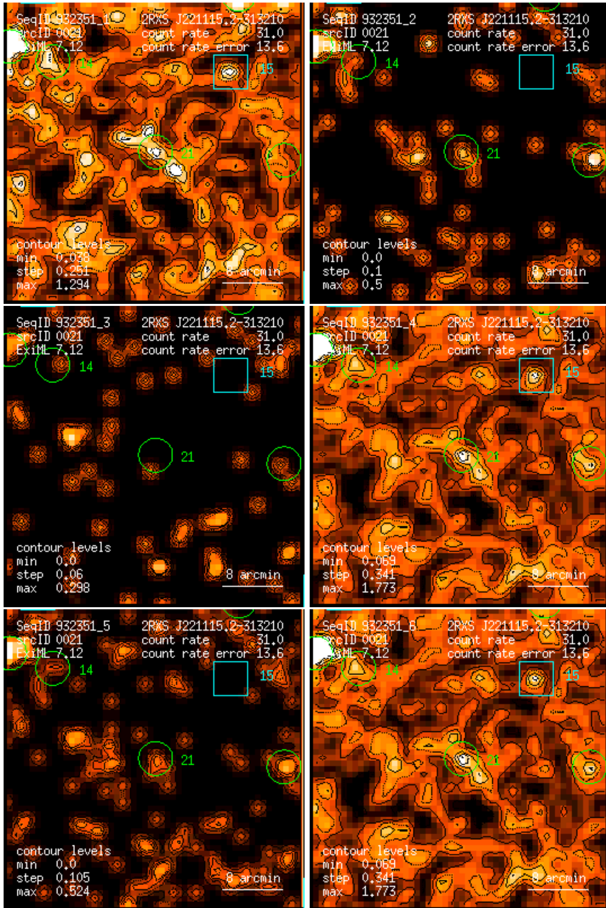
Figure 21: RASS 932351: detection 0021: band rate images, Gaussian filter: (1) PSPC channels 11 – 41, (2) 52 – 90, (3) 91 – 201, (4) 11 – 235, (5) 52 – 201, (6) 11 – 201. Broad band rates in counts/ks. Band rate contour levels in counts/ks/arcmin 2 .
